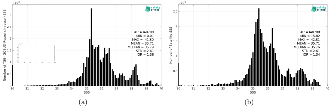
Figure 2: Histograms of SSS from TSG (GOSUD-Research-vessel) (a) and SMOS SSS L3 v8 - 18 Days (CATDS-CEC-LOCEAN) (b) considering all match-up pairs per bins of 0.1 over the Mid-Low Latitudes 45N-45S Pi-MEP region and for the full satellite product period.
