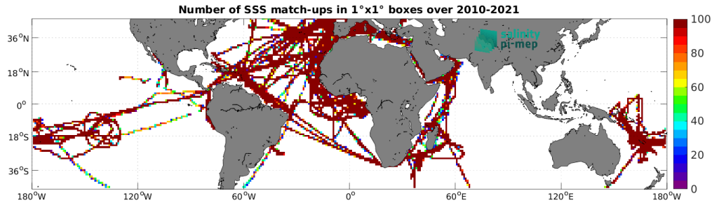
Figure 4: Number of SSS match-ups between TSG (GOSUD-Research-vessel) SSS and the SMOS SSS L3 v8 - 18 Days (CATDS-CEC-LOCEAN) SSS product for the Mid-Low Latitudes 45N-45S Pi-MEP region over 1^\circ \times 1^\circ boxes and for the full satellite product period.
