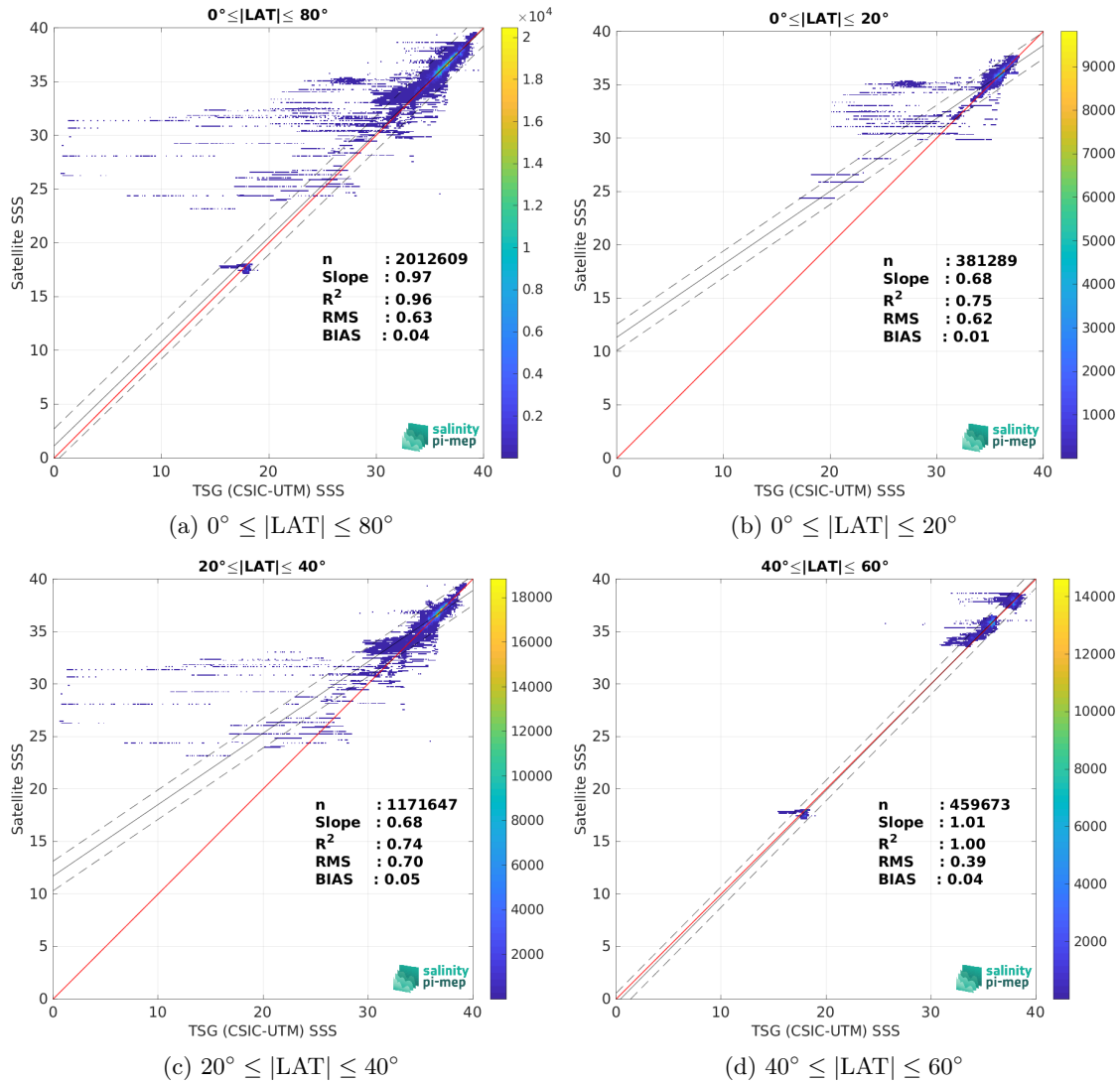
Figure 9: Contour maps of the concentration of SMOS SSS L3 v8 - 18 Days (CATDS-CEC-LOCEAN) SSS (y-axis) versus TSG (CSIC-UTM) SSS (x-axis) at match-up pairs for different latitude bands. For each plot, the red line shows x=y . The black thin and dashed lines indicate a linear fit through the data cloud and the \pm 95\% confidence levels, respectively. The number match-up pairs n , the slope and R^2 coefficient of the linear fit, the root mean square (RMS) and the mean bias between satellite and in situ data are indicated for each latitude band in each plots.
