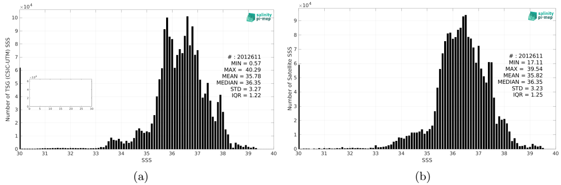
Figure 2: Histograms of SSS from TSG (CSIC-UTM) (a) and SMOS SSS L3 v8 - 18 Days (CATDS-CEC-LOCEAN) (b) considering all match-up pairs per bins of 0.1 over the Mid-Low Latitudes 45N-45S Pi-MEP region and for the full satellite product period.
