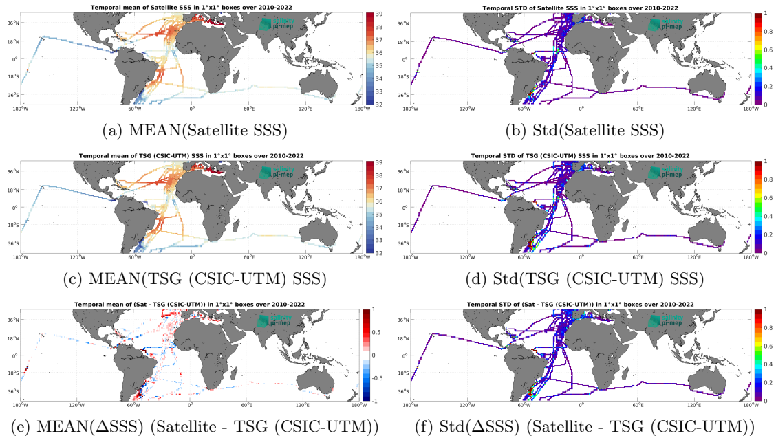
Figure 6: Temporal mean (left) and Std (right) of SSS from SMOS SSS L3 v8 - 18 Days (CATDS-CEC-LOCEAN) (top), TSG (CSIC-UTM) (middle), and of \Delta SSS (Satellite - TSG (CSIC-UTM)). Only match-up pairs are used to generate these maps.
