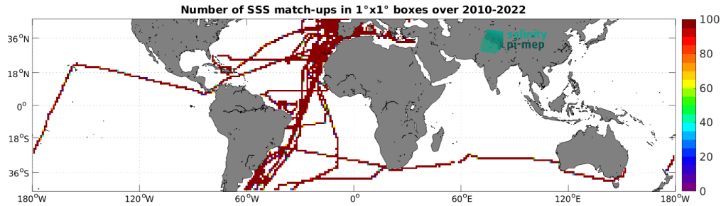
Figure 4: Number of SSS match-ups between TSG (CSIC-UTM) SSS and the SMOS SSS L3 v8 - 18 Days (CATDS-CEC-LOCEAN) SSS product for the Mid-Low Latitudes 45N-45S Pi-MEP region over 1^\circ \times 1^\circ boxes and for the full satellite product period.
