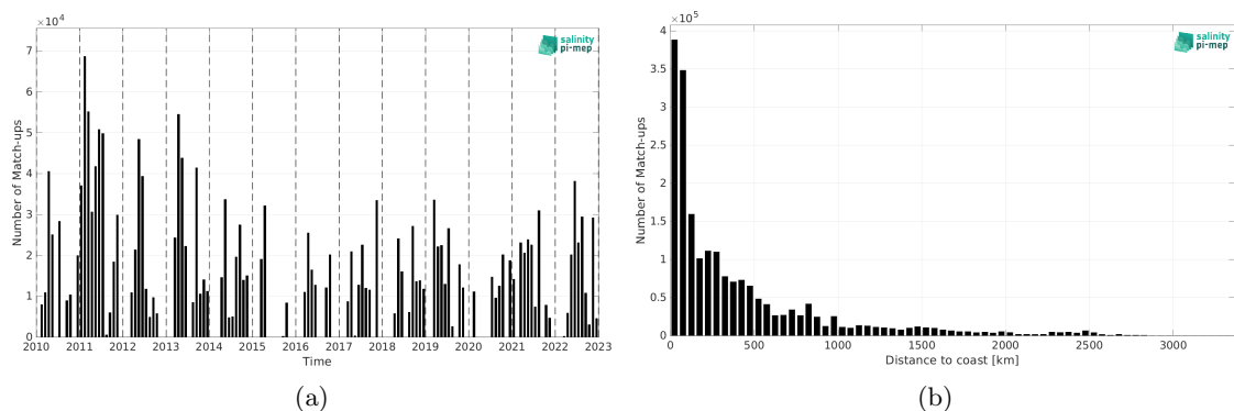
Figure 1: Number of match-ups between TSG (CSIC-UTM) and SMOS SSS L3 v8 - 18 Days (CATDS-CEC-LOCEAN) SSS as a function of time (a) and as function of the distance to coast (b) over the Mid-Low Latitudes 45N-45S Pi-MEP region and for the full satellite product period.
