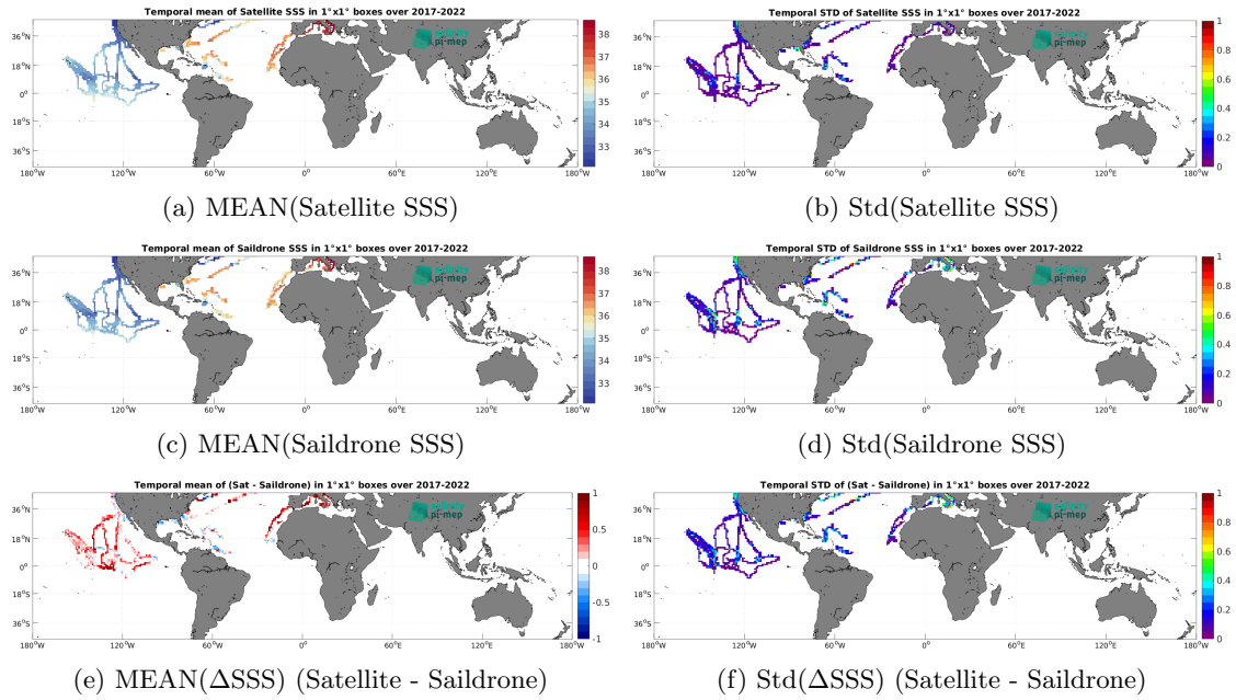
Figure 6: Temporal mean (left) and Std (right) of SSS from SMOS SSS L3 v8 - 18 Days (CATDS-CEC-LOCEAN) (top), Saildrone (middle), and of \Delta SSS (Satellite - Saildrone). Only match-up pairs are used to generate these maps.
