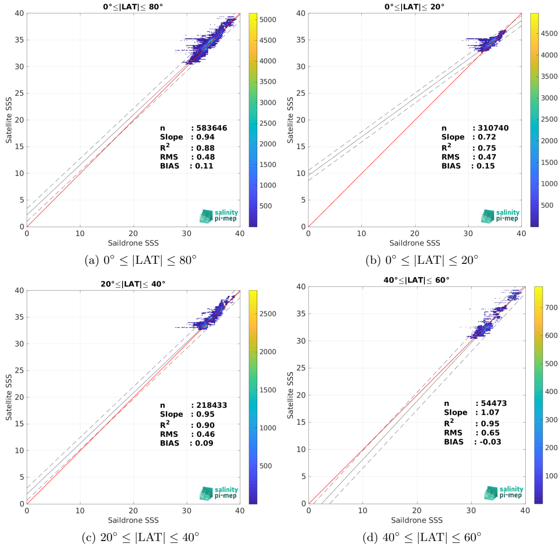
Figure 9: Contour maps of the concentration of SMOS SSS L3 v8 - 18 Days (CATDS-CEC-LOCEAN) SSS (y-axis) versus Sairdrone SSS (x-axis) at match-up pairs for different latitude bands. For each plot, the red line shows x=y . The black thin and dashed lines indicate a linear fit through the data cloud and the \pm 95\% confidence levels, respectively. The number match-up pairs n , the slope and R^2 coefficient of the linear fit, the root mean square (RMS) and the mean bias between satellite and in situ data are indicated for each latitude band in each plots.
