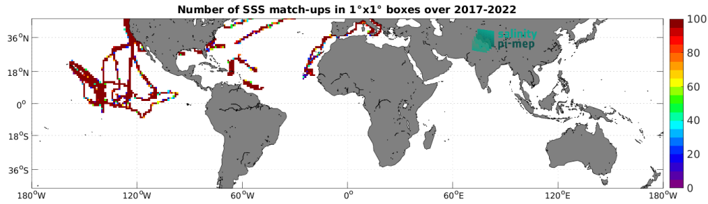
Figure 4: Number of SSS match-ups between Saildrone SSS and the SMOS SSS L3 v8 - 18 Days (CATDS-CEC-LOCEAN) SSS product for the Mid-Low Latitudes 45N-45S Pi-MEP region over 1^\circ \times 1^\circ boxes and for the full satellite product period.
