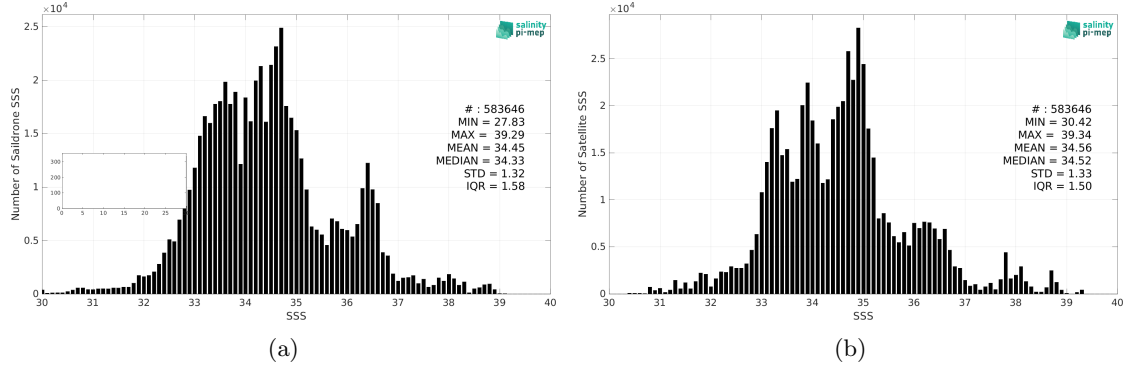
Figure 2: Histograms of SSS from Saildrone (a) and SMOS SSS L3 v8 - 18 Days (CATDS-CEC-LOCEAN) (b) considering all match-up pairs per bins of 0.1 over the Mid-Low Latitudes 45N-45S Pi-MEP region and for the full satellite product period.
