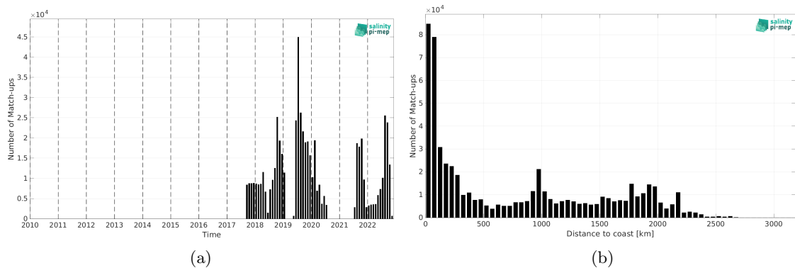
Figure 1: Number of match-ups between Saildrone and SMOS SSS L3 v8 - 18 Days (CATDS-CEC-LOCEAN) SSS as a function of time (a) and as function of the distance to coast (b) over the Mid-Low Latitudes 45N-45S Pi-MEP region and for the full satellite product period.
