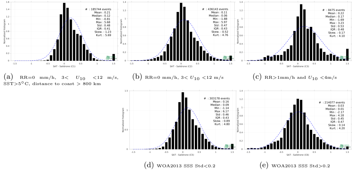
Figure 13: Normalized histogram of \Delta SSS (SMOS SSS L3 v8 - 18 Days (CATDS-CECOS-LOCEAN) - Saildrone) for 5 different subdatasets corresponding to: RR=0 mm/h, 3 < U_{10} < 12 m/s, SST>5°C, distance to coast > 800 km (a), RR=0 mm/h, 3 < U_{10} < 12 m/s (b), RR>1mm/h and U_{10} < 4 m/s (c), WOA2013 SSS Std<0.2 (d), WOA2013 SSS Std>0.2 (e).
