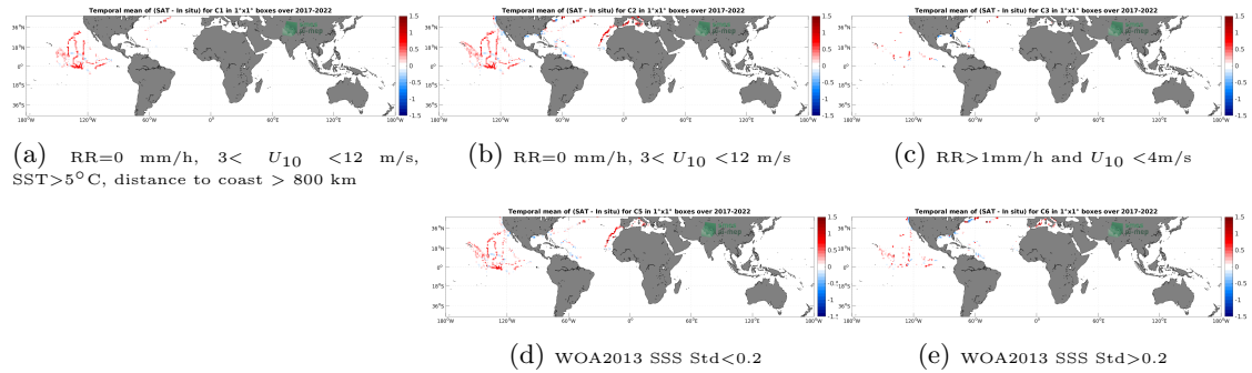
Figure 12: Temporal mean gridded over spatial boxes of size 1^\circ \times 1^\circ of \Delta SSS (SMOS SSS L3 v8 - 18 Days (CATDS-CECOS-LOCEAN) - Sairdrone) for 5 different subdatasets corresponding to: RR=0 mm/h, 3 < U_{10} < 12 m/s, SST > 5^\circ\text{C} , distance to coast > 800 km (a), RR=0 mm/h, 3 < U_{10} < 12 m/s (b), RR > 1 mm/h and U_{10} < 4 m/s (c), WOA2013 SSS Std < 0.2 (d), WOA2013 SSS Std > 0.2 (e).
