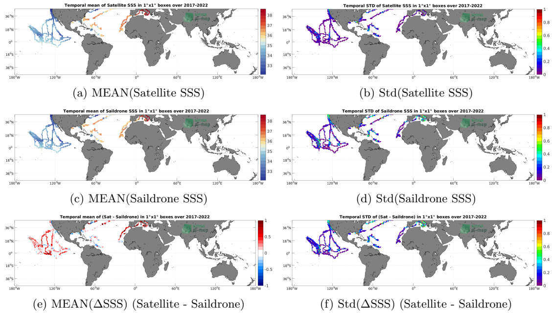
Figure 6: Temporal mean (left) and Std (right) of SSS from SMOS SSS L3 v8 - 18 Days (CATDS-CECOS-LOCEAN) (top), Saildrone (middle), and of \Delta SSS (Satellite - Saildrone). Only match-up pairs are used to generate these maps.
