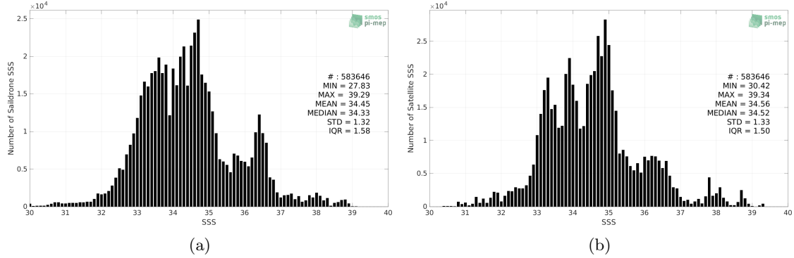
Figure 2: Histograms of SSS from Saildrone (a) and SMOS SSS L3 v8 - 18 Days (CATDS-CECOS-LOCEAN) (b) considering all match-up pairs per bins of 0.1 over the Mid-Low Latitudes 45N-45S Pi-MEP region and for the full satellite product period.
