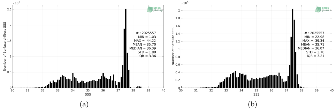
Figure 2: Histograms of SSS from Surface drifters (a) and SMOS SSS L3 v8 - 18 Days (CATDS-CECOS-LOCEAN) (b) considering all match-up pairs per bins of 0.1 over the Mid-Low Latitudes 45N-45S Pi-MEP region and for the full satellite product period.
