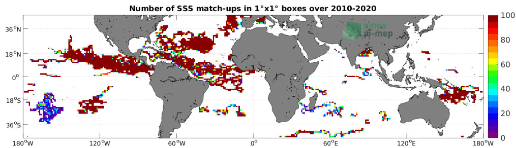
Figure 3: Number of SSS match-ups between Surface drifters SSS and the SMOS SSS L3 v8 - 18 Days (CATDS-CECOS-LOCEAN) SSS product for the Mid-Low Latitudes 45N-45S Pi-MEP region over 1^\circ \times 1^\circ boxes and for the full satellite product period.
