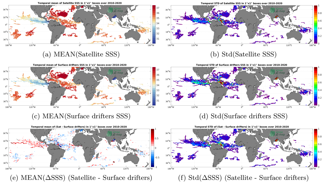
Figure 5: Temporal mean (left) and Std (right) of SSS from SMOS SSS L3 v8 - 18 Days (CATDS-CECOS-LOCEAN) (top), Surface drifters (middle), and of \Delta SSS (Satellite - Surface drifters). Only match-up pairs are used to generate these maps.
