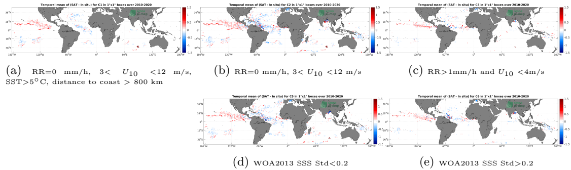
Figure 11: Temporal mean gridded over spatial boxes of size 1^\circ \times 1^\circ of \Delta SSS (SMOS SSS L3 v8 - 18 Days (CATDS-CECOS-LOCEAN) - Surface drifters) for 5 different subdatasets corresponding to:RR=0 mm/h, 3 < U_{10} < 12 m/s, SST >5^\circ C, distance to coast > 800 km (a), RR=0 mm/h, 3 < U_{10} < 12 m/s (b), RR >1 mm/h and U_{10} < 4 m/s (c), WOA2013 SSS Std <0.2 (d), WOA2013 SSS Std >0.2 (e).
