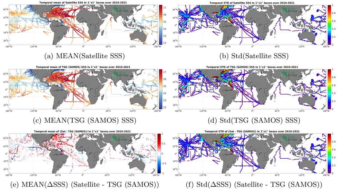
Figure 6: Temporal mean (left) and Std (right) of SSS from SMOS SSS L3 v7 - 9 Days (CATDS-CECOS-LOCEAN) (top), TSG (SAMOS) (middle), and of \Delta SSS (Satellite - TSG (SAMOS)). Only match-up pairs are used to generate these maps.
