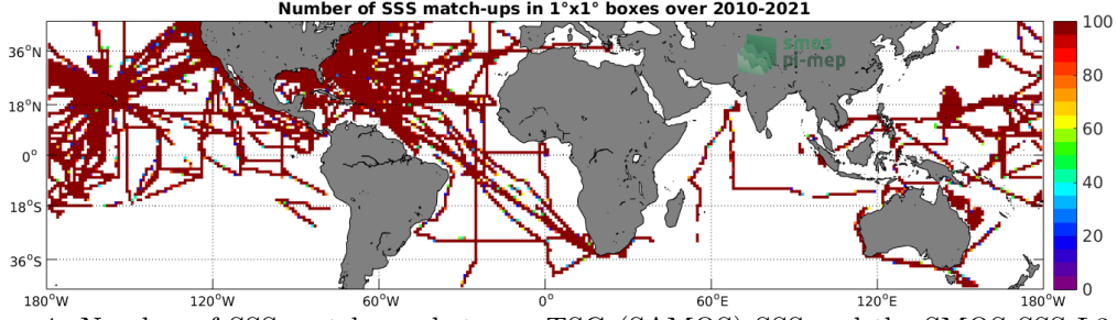
Figure 4: Number of SSS match-ups between TSG (SAMOS) SSS and the SMOS SSS L3 v7 - 9 Days (CATDS-CECOS-LOCEAN) SSS product for the Mid-Low Latitudes 45N-45S Pi-MEP region over 1^\circ \times 1^\circ boxes and for the full satellite product period.
