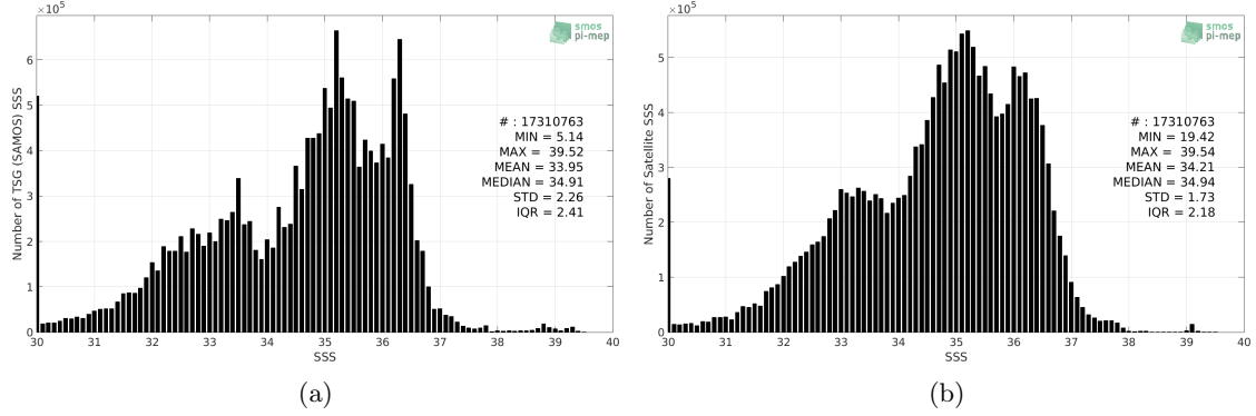
Figure 2: Histograms of SSS from TSG (SAMOS) (a) and SMOS SSS L3 v7 - 9 Days (CATDS-CECOS-LOCEAN) (b) considering all match-up pairs per bins of 0.1 over the Mid-Low Latitudes 45N-45S Pi-MEP region and for the full satellite product period.
