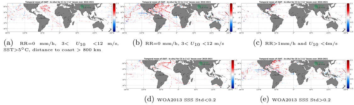
Figure 12: Temporal mean gridded over spatial boxes of size 1^\circ \times 1^\circ of \Delta SSS (SMOS SSS L3 v7 - 9 Days (CATDS-CECOS-LOCEAN) - TSG (SAMOS)) for 5 different subdatasets corresponding to: RR=0 mm/h, 3 < U_{10} < 12 m/s, SST > 5^\circ C , distance to coast > 800 km (a), RR=0 mm/h, 3 < U_{10} < 12 m/s (b), RR > 1 mm/h and U_{10} < 4 m/s (c), WOA2013 SSS Std < 0.2 (d), WOA2013 SSS Std > 0.2 (e).
