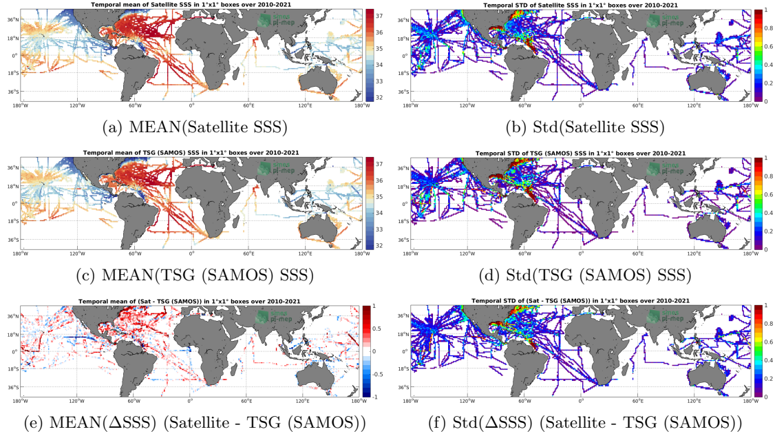
Figure 6: Temporal mean (left) and Std (right) of SSS from SMOS SSS L3 v7 - 9 Days (CATDS-CECOS-LOCEAN) (top), TSG (SAMOS) (middle), and of \Delta SSS (Satellite - TSG (SAMOS)). Only match-up pairs are used to generate these maps.
