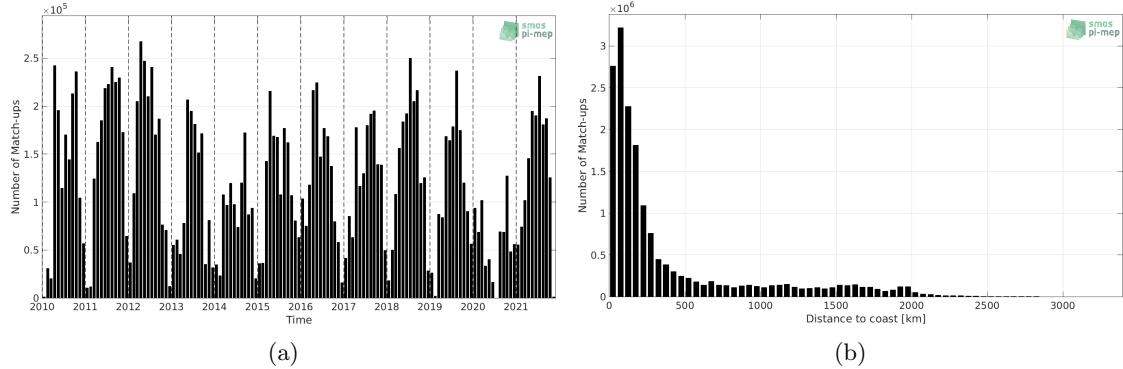
Figure 1: Number of match-ups between TSG (SAMOS) and SMOS SSS L3 v7 - 9 Days (CATDS-CECOS-LOCEAN) SSS as a function of time (a) and as function of the distance to coast (b) over the Mid-Low Latitudes 45N-45S Pi-MEP region and for the full satellite product period.
