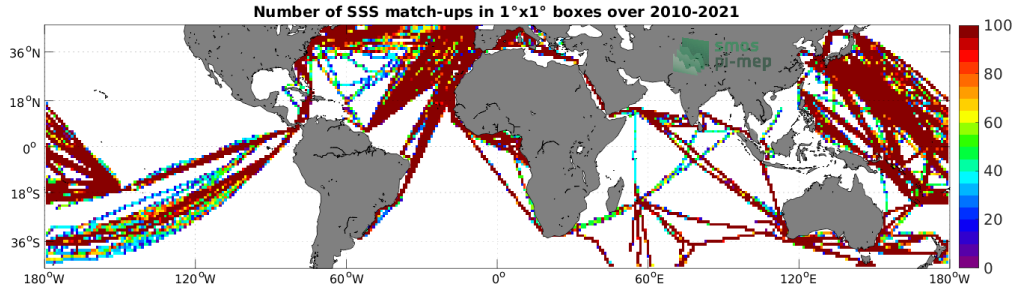
Figure 4: Number of SSS match-ups between TSG (LEGOS-DM) SSS and the SMOS SSS L3 v7 - 9 Days (CATDS-CECOS-LOCEAN) SSS product for the Mid-Low Latitudes 45N-45S Pi-MEP region over 1^{\circ} \times 1^{\circ} boxes and for the full satellite product period.
