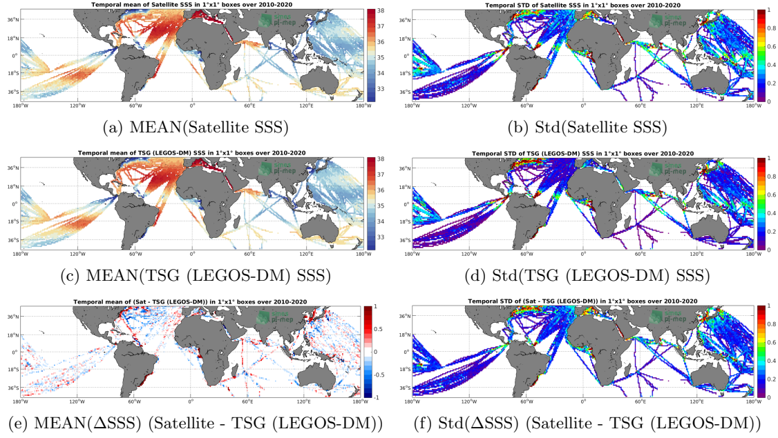
Figure 6: Temporal mean (left) and Std (right) of SSS from SMOS SSS L3 v7 - 9 Days (CATDS-CECOS-LOCEAN) (top), TSG (LEGOS-DM) (middle), and of \Delta SSS (Satellite - TSG (LEGOS-DM)). Only match-up pairs are used to generate these maps.
