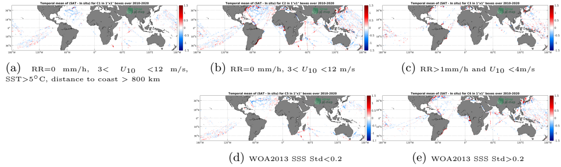
Figure 12: Temporal mean gridded over spatial boxes of size 1^\circ \times 1^\circ of \Delta SSS (SMOS SSS L3 v7 - 9 Days (CATDS-CECOS-LOCEAN) - TSG (LEGOS-DM)) for 5 different subdatasets corresponding to: RR=0 mm/h, 3 < U_{10} < 12 m/s, SST > 5^\circ C , distance to coast > 800 km (a), RR=0 mm/h, 3 < U_{10} < 12 m/s (b), RR > 1 mm/h and U_{10} < 4 m/s (c), WOA2013 SSS Std < 0.2 (d), WOA2013 SSS Std > 0.2 (e).
