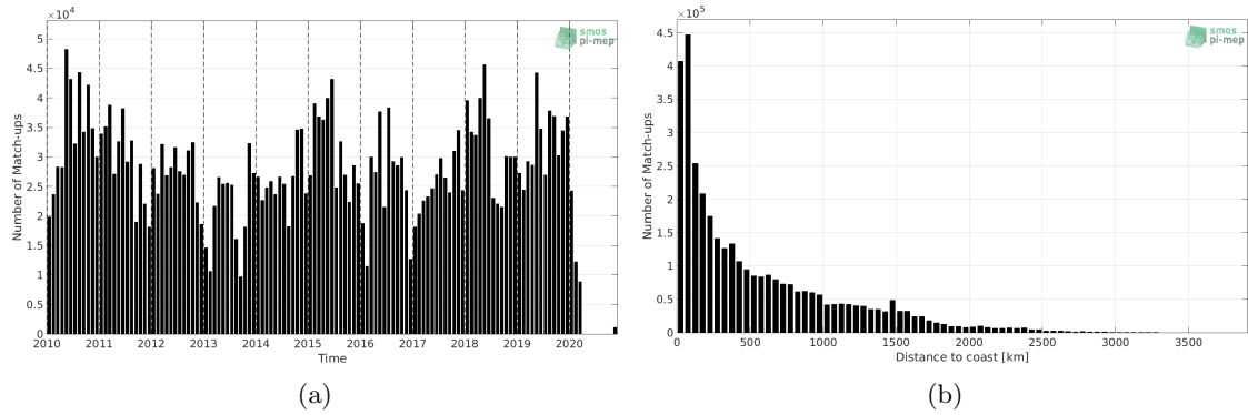
Figure 1: Number of match-ups between TSG (LEGOS-DM) and SMOS SSS L3 v7 - 9 Days (CATDS-CECOS-LOCEAN) SSS as a function of time (a) and as function of the distance to coast (b) over the Mid-Low Latitudes 45N-45S Pi-MEP region and for the full satellite product period.
