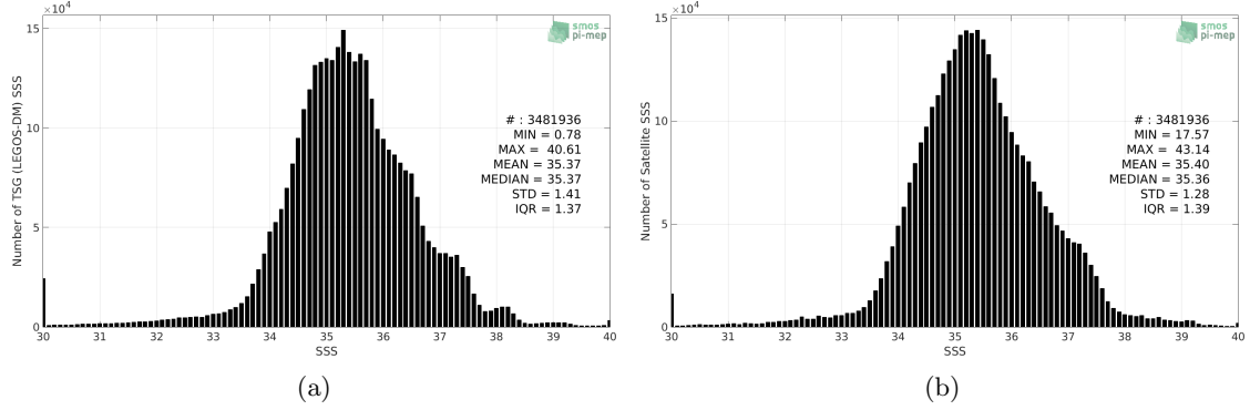
Figure 2: Histograms of SSS from TSG (LEGOS-DM) (a) and SMOS SSS L3 v7 - 9 Days (CATDS-CECOS-LOCEAN) (b) considering all match-up pairs per bins of 0.1 over the Mid-Low Latitudes 45N-45S Pi-MEP region and for the full satellite product period.
