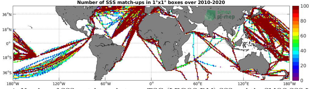
Figure 4: Number of SSS match-ups between TSG (LEGOS-DM) SSS and the SMOS SSS L3 v7 - 9 Days (CATDS-CECOS-LOCEAN) SSS product for the Mid-Low Latitudes 45N-45S Pi-MEP region over 1^\circ \times 1^\circ boxes and for the full satellite product period.
