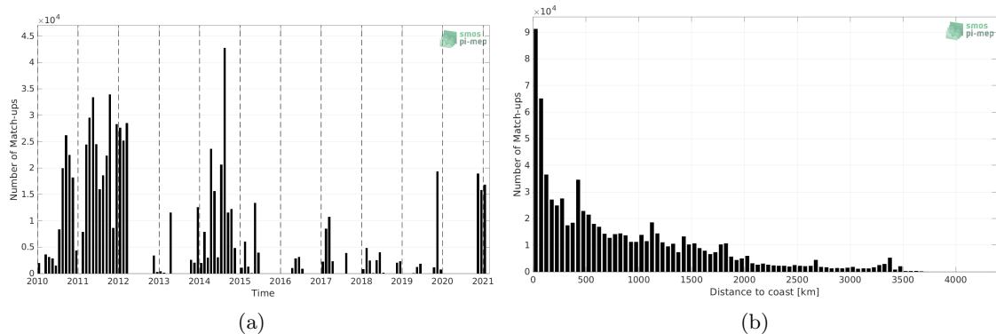
Figure 1: Number of match-ups between TSG (GOSUD-Sailing-ship) and SMOS SSS L3 v7 - 9 Days (CATDS-CECOS-LOCEAN) SSS as a function of time (a) and as function of the distance to coast (b) over the Mid-Low Latitudes 45N-45S Pi-MEP region and for the full satellite product period.
