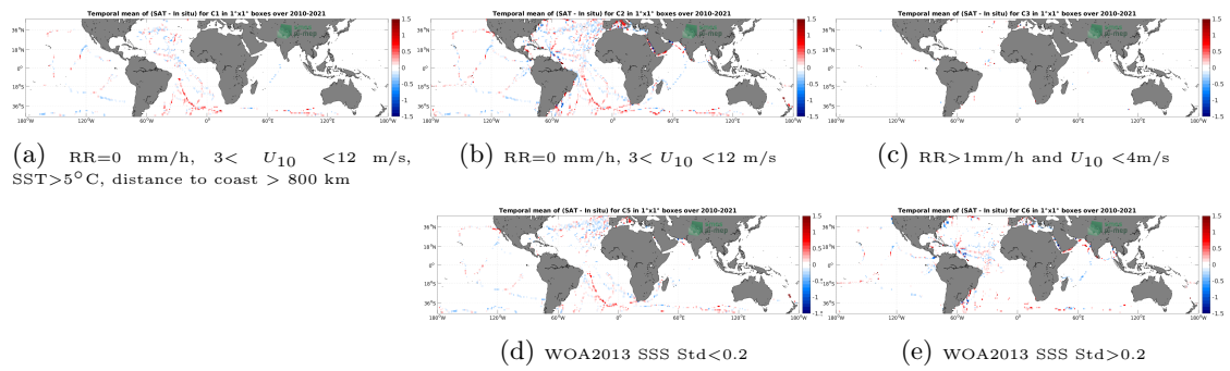
Figure 12: Temporal mean gridded over spatial boxes of size 1^\circ \times 1^\circ of \Delta SSS (SMOS SSS L3 v7 - 9 Days (CATDS-CECOS-LOCEAN) - TSG (GOSUD-Sailing-ship)) for 5 different subdatasets corresponding to: RR=0 mm/h, 3 < U_{10} < 12 m/s, SST > 5°C, distance to coast > 800 km (a), RR=0 mm/h, 3 < U_{10} < 12 m/s (b), RR > 1mm/h and U_{10} < 4 m/s (c), WOA2013 SSS Std < 0.2 (d), WOA2013 SSS Std > 0.2 (e).
