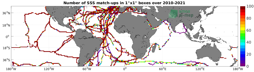
Figure 4: Number of SSS match-ups between TSG (GOSUD-Sailing-ship) SSS and the SMOS SSS L3 v7 - 9 Days (CATDS-CECOS-LOCEAN) SSS product for the Mid-Low Latitudes 45N-45S Pi-MEP region over 1^\circ \times 1^\circ boxes and for the full satellite product period.
