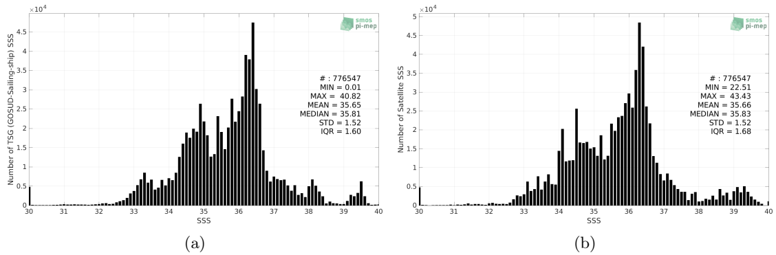
Figure 2: Histograms of SSS from TSG (GOSUD-Sailing-ship) (a) and SMOS SSS L3 v7 - 9 Days (CATDS-CECOS-LOCEAN) (b) considering all match-up pairs per bins of 0.1 over the Mid-Low Latitudes 45N-45S Pi-MEP region and for the full satellite product period.
