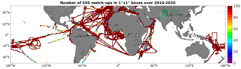
Figure 4: Number of SSS match-ups between TSG (GOSUD-Research-vessel) SSS and the SMOS SSS L3 v7 - 9 Days (CATDS-CECOS-LOCEAN) SSS product for the Mid-Low Latitudes 45N-45S Pi-MEP region over 1^\circ \times 1^\circ boxes and for the full satellite product period.
