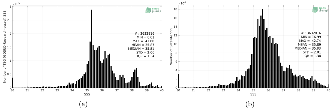
Figure 2: Histograms of SSS from TSG (GOSUD-Research-vessel) (a) and SMOS SSS L3 v7 - 9 Days (CATDS-CECOS-LOCEAN) (b) considering all match-up pairs per bins of 0.1 over the Mid-Low Latitudes 45N-45S Pi-MEP region and for the full satellite product period.
