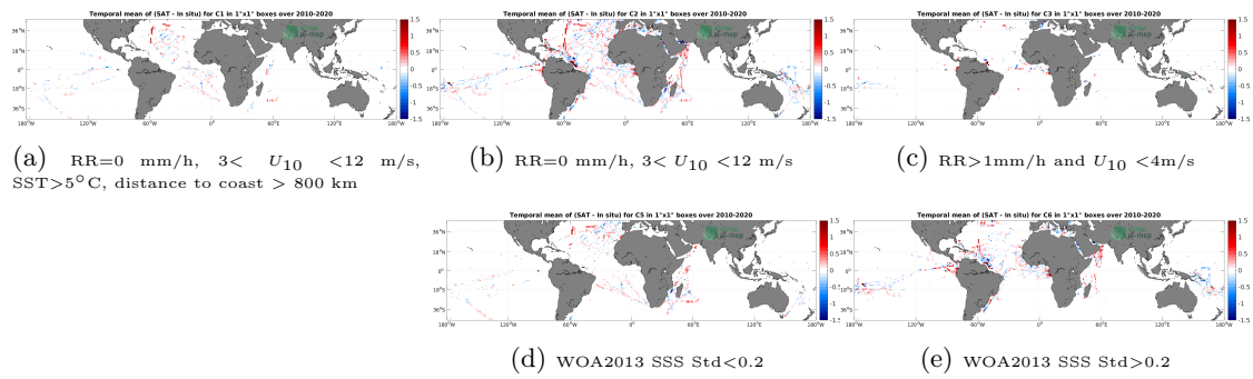
Figure 12: Temporal mean gridded over spatial boxes of size 1^\circ \times 1^\circ of \Delta\text{SSS} (SMOS SSS L3 v7 - 9 Days (CATDS-CECOS-LOCEAN) - TSG (GOSUD-Research-vessel)) for 5 different subdatasets corresponding to: RR=0 mm/h, 3 < U_{10} < 12 m/s, SST>5°C, distance to coast > 800 km (a), RR=0 mm/h, 3 < U_{10} < 12 m/s (b), RR>1mm/h and U_{10} < 4 m/s (c), WOA2013 SSS Std<0.2 (d), WOA2013 SSS Std>0.2 (e).
