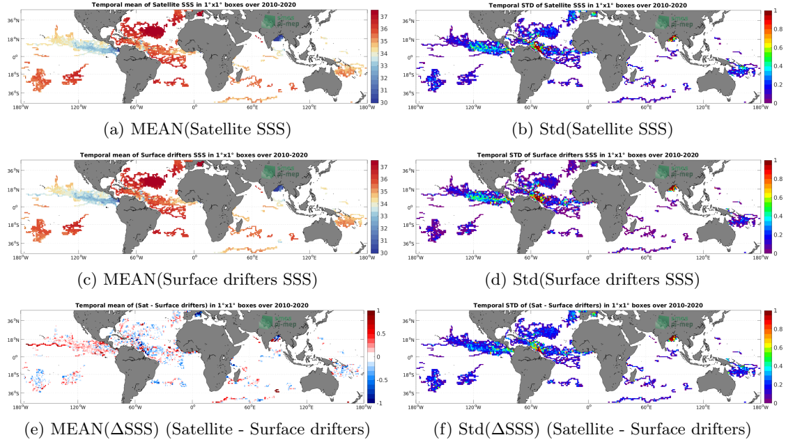
Figure 5: Temporal mean (left) and Std (right) of SSS from SMOS SSS L3 v7 - 9 Days (CATDS-CECOS-LOCEAN) (top), Surface drifters (middle), and of \Delta SSS (Satellite - Surface drifters). Only match-up pairs are used to generate these maps.
