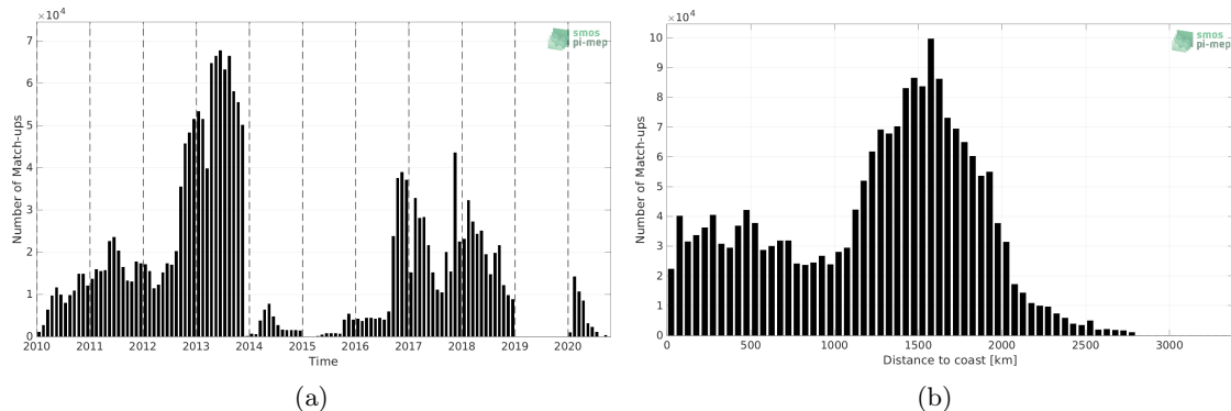
Figure 1: Number of match-ups between Surface drifters and SMOS SSS L3 v7 - 9 Days (CATDS-CECOS-LOCEAN) SSS as a function of time (a) and as function of the distance to coast (b) over the Mid-Low Latitudes 45N-45S Pi-MEP region and for the full satellite product period.
