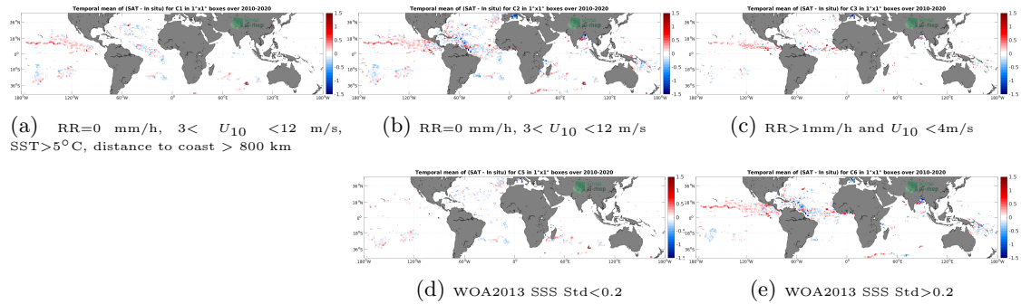
Figure 11: Temporal mean gridded over spatial boxes of size 1^\circ \times 1^\circ of \Delta SSS (SMOS SSS L3 v7 - 9 Days (CATDS-CECOS-LOCEAN) - Surface drifters) for 5 different subdatasets corresponding to:RR=0 mm/h, 3 < U_{10} < 12 m/s, SST >5^\circ C, distance to coast > 800 km (a), RR=0 mm/h, 3 < U_{10} < 12 m/s (b), RR >1 mm/h and U_{10} < 4 m/s (c), WOA2013 SSS Std <0.2 (d), WOA2013 SSS Std >0.2 (e).
