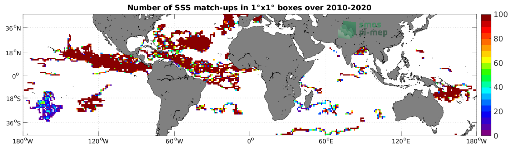
Figure 3: Number of SSS match-ups between Surface drifters SSS and the SMOS SSS L3 v7 - 9 Days (CATDS-CECOS-LOCEAN) SSS product for the Mid-Low Latitudes 45N-45S Pi-MEP region over 1^\circ \times 1^\circ boxes and for the full satellite product period.
