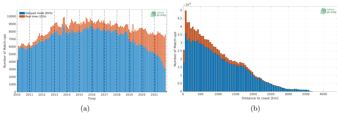
Figure 1: Number of match-ups between Argo and SMOS SSS L3 v7 - 9 Days (CATDS-CECOS-LOCEAN) SSS as a function of time (a) and as function of the distance to coast (b) over the Mid-Low Latitudes 45N-45S Pi-MEP region and for the full satellite product period.
