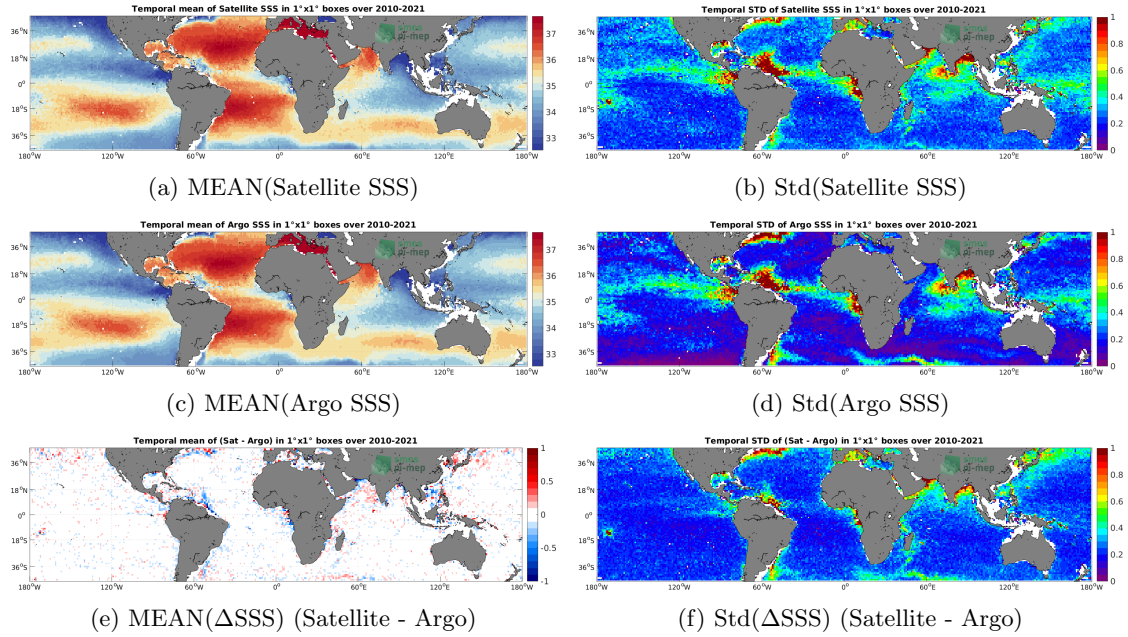
Figure 6: Temporal mean (left) and Std (right) of SSS from SMOS SSS L3 v7 - 9 Days (CATDS-CECOS-LOCEAN) (top), Argo (middle), and of \Delta SSS (Satellite - Argo). Only match-up pairs are used to generate these maps.
