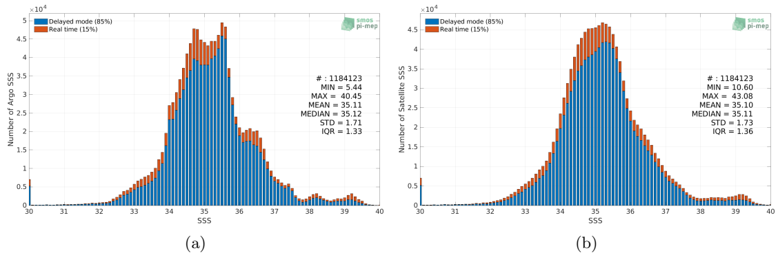
Figure 2: Histograms of SSS from Argo (a) and SMOS SSS L3 v7 - 9 Days (CATDS-CECOS-LOCEAN) (b) considering all match-up pairs per bins of 0.1 over the Mid-Low Latitudes 45N-45S Pi-MEP region and for the full satellite product period.
