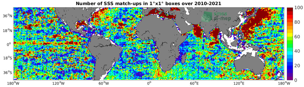
Figure 4: Number of SSS match-ups between Argo SSS and the SMOS SSS L3 v7 - 9 Days (CATDS-CECOS-LOCEAN) SSS product for the Mid-Low Latitudes 45N-45S Pi-MEP region over 1^\circ \times 1^\circ boxes and for the full satellite product period.
