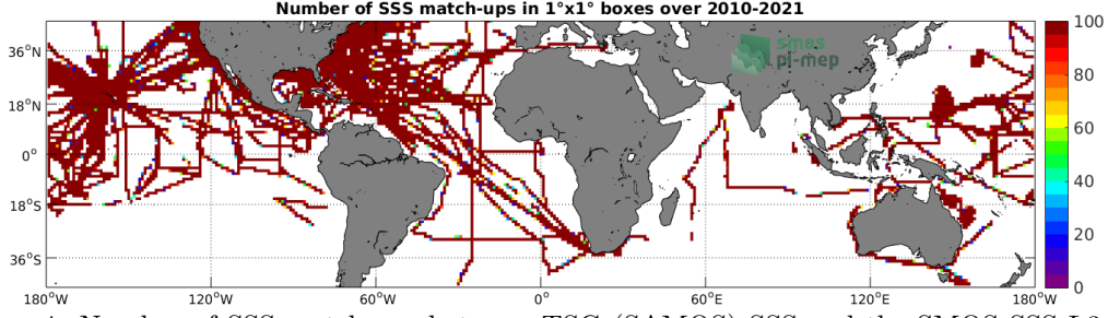
Figure 4: Number of SSS match-ups between TSG (SAMOS) SSS and the SMOS SSS L3 v7 - 18 Days (CATDS-CECOS-LOCEAN) SSS product for the Mid-Low Latitudes 45N-45S Pi-MEP region over 1^\circ \times 1^\circ boxes and for the full satellite product period.
