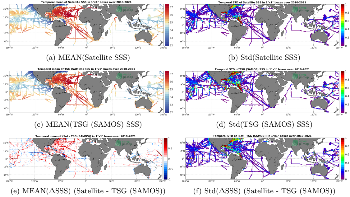
Figure 6: Temporal mean (left) and Std (right) of SSS from SMOS SSS L3 v7 - 18 Days (CATDS-CECOS-LOCEAN) (top), TSG (SAMOS) (middle), and of \Delta SSS (Satellite - TSG (SAMOS)). Only match-up pairs are used to generate these maps.
