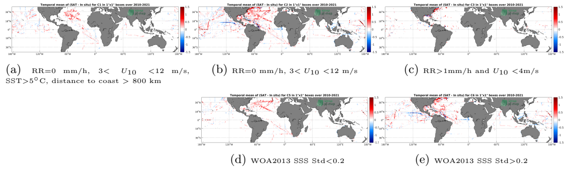
Figure 12: Temporal mean gridded over spatial boxes of size 1^\circ \times 1^\circ of \Delta SSS (SMOS SSS L3 v7 - 18 Days (CATDS-CECOS-LOCEAN) - TSG (SAMOS)) for 5 different subdatasets corresponding to: RR=0 mm/h, 3 < U_{10} < 12 m/s, SST > 5^\circ C , distance to coast > 800 km (a), RR=0 mm/h, 3 < U_{10} < 12 m/s (b), RR > 1 mm/h and U_{10} < 4 m/s (c), WOA2013 SSS Std < 0.2 (d), WOA2013 SSS Std > 0.2 (e).
