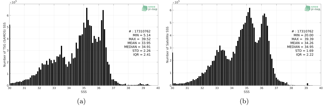
Figure 2: Histograms of SSS from TSG (SAMOS) (a) and SMOS SSS L3 v7 - 18 Days (CATDS-CECOS-LOCEAN) (b) considering all match-up pairs per bins of 0.1 over the Mid-Low Latitudes 45N-45S Pi-MEP region and for the full satellite product period.
