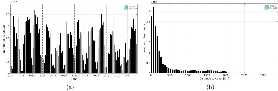
Figure 1: Number of match-ups between TSG (SAMOS) and SMOS SSS L3 v7 - 18 Days (CATDS-CECOS-LOCEAN) SSS as a function of time (a) and as function of the distance to coast (b) over the Mid-Low Latitudes 45N-45S Pi-MEP region and for the full satellite product period.
