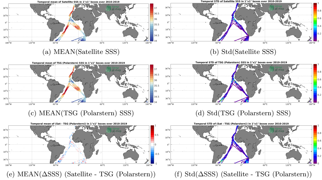
Figure 6: Temporal mean (left) and Std (right) of SSS from SMOS SSS L3 v7 - 18 Days (CATDS-CECOS-LOCEAN) (top), TSG (Polarstern) (middle), and of \Delta SSS (Satellite - TSG (Polarstern)). Only match-up pairs are used to generate these maps.
