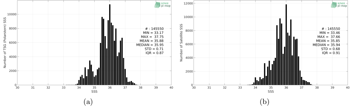
Figure 2: Histograms of SSS from TSG (Polarstern) (a) and SMOS SSS L3 v7 - 18 Days (CATDS-CECOS-LOCEAN) (b) considering all match-up pairs per bins of 0.1 over the Mid-Low Latitudes 45N-45S Pi-MEP region and for the full satellite product period.
