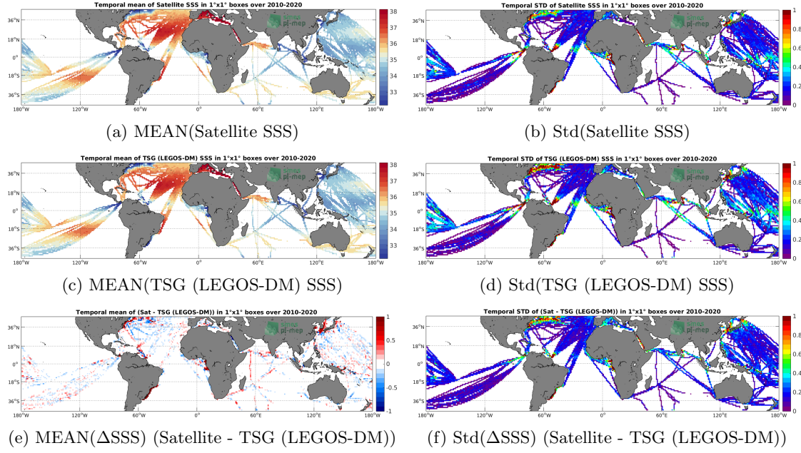
Figure 6: Temporal mean (left) and Std (right) of SSS from SMOS SSS L3 v7 - 18 Days (CATDS-CECOS-LOCEAN) (top), TSG (LEGOS-DM) (middle), and of \Delta SSS (Satellite - TSG (LEGOS-DM)). Only match-up pairs are used to generate these maps.
