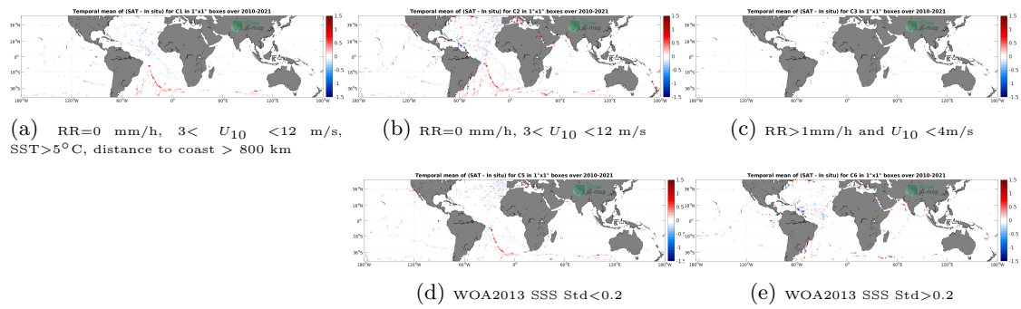
Figure 12: Temporal mean gridded over spatial boxes of size 1^\circ \times 1^\circ of \Delta\text{SSS} (SMOS SSS L3 v7 - 18 Days (CATDS-CECOS-LOCEAN) - TSG (GOSUD-Sailing-ship)) for 5 different subdatasets corresponding to: RR=0 mm/h, 3 < U_{10} < 12 m/s, SST > 5°C, distance to coast > 800 km (a), RR=0 mm/h, 3 < U_{10} < 12 m/s (b), RR > 1mm/h and U_{10} < 4 m/s (c), WOA2013 SSS Std < 0.2 (d), WOA2013 SSS Std > 0.2 (e).
