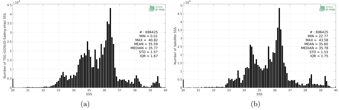
Figure 2: Histograms of SSS from TSG (GOSUD-Sailing-ship) (a) and SMOS SSS L3 v7 - 18 Days (CATDS-CECOS-LOCEAN) (b) considering all match-up pairs per bins of 0.1 over the Mid-Low Latitudes 45N-45S Pi-MEP region and for the full satellite product period.
