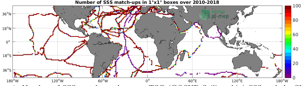
Figure 4: Number of SSS match-ups between TSG (GOSUD-Sailing-ship) SSS and the SMOS SSS L3 v7 - 18 Days (CATDS-CECOS-LOCEAN) SSS product for the Mid-Low Latitudes 45N-45S Pi-MEP region over 1^\circ \times 1^\circ boxes and for the full satellite product period.
