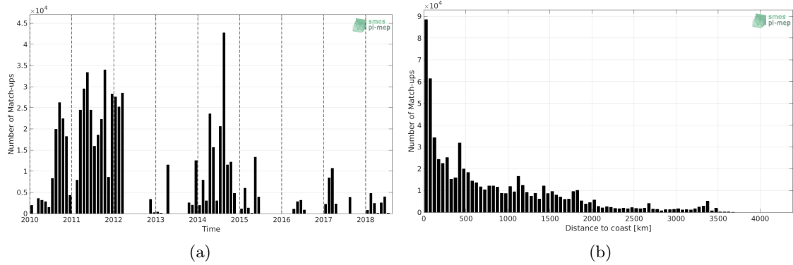
Figure 1: Number of match-ups between TSG (GOSUD-Sailing-ship) and SMOS SSS L3 v7 - 18 Days (CATDS-CECOS-LOCEAN) SSS as a function of time (a) and as function of the distance to coast (b) over the Mid-Low Latitudes 45N-45S Pi-MEP region and for the full satellite product period.
