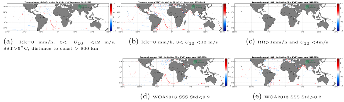
Figure 12: Temporal mean gridded over spatial boxes of size 1^\circ \times 1^\circ of \Delta SSS (SMOS SSS L3 v7 - 18 Days (CATDS-CECOS-LOCEAN) - TSG (GOSUD-Sailing-ship)) for 5 different subdatasets corresponding to: RR=0 mm/h, 3 < U_{10} < 12 m/s, SST > 5^\circ C , distance to coast > 800 km (a), RR=0 mm/h, 3 < U_{10} < 12 m/s (b), RR > 1 mm/h and U_{10} < 4 m/s (c), WOA2013 SSS Std < 0.2 (d), WOA2013 SSS Std > 0.2 (e).
