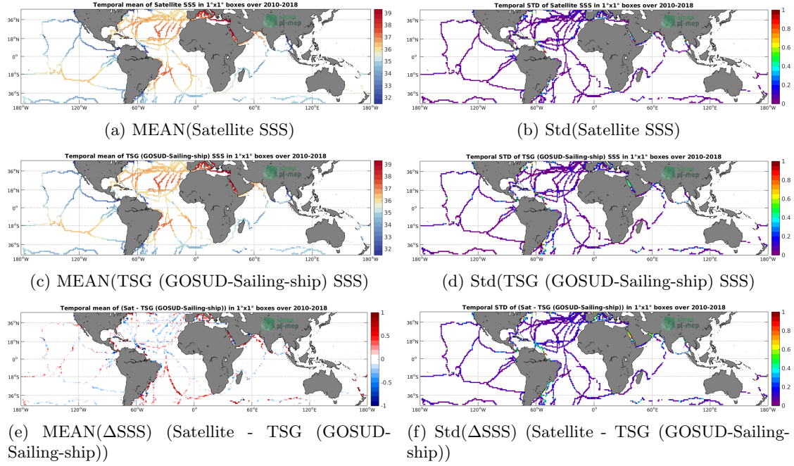
Figure 6: Temporal mean (left) and Std (right) of SSS from SMOS SSS L3 v7 - 18 Days (CATDS-CECOS-LOCEAN) (top), TSG (GOSUD-Sailing-ship) (middle), and of \Delta SSS (Satellite - TSG (GOSUD-Sailing-ship)). Only match-up pairs are used to generate these maps.
