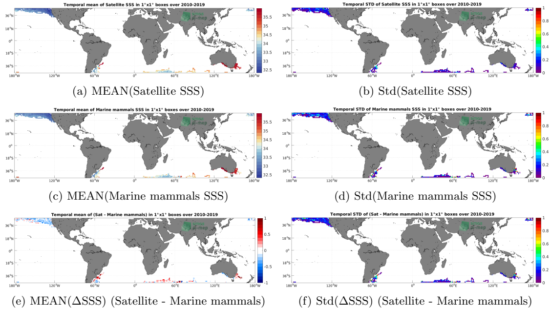
Figure 6: Temporal mean (left) and Std (right) of SSS from SMOS SSS L3 v7 - 18 Days (CATDS-CECOS-LOCEAN) (top), Marine mammals (middle), and of \Delta SSS (Satellite - Marine mammals). Only match-up pairs are used to generate these maps.
