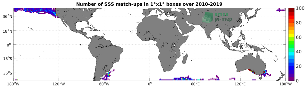
Figure 4: Number of SSS match-ups between Marine mammals SSS and the SMOS SSS L3 v7 - 18 Days (CATDS-CECOS-LOCEAN) SSS product for the Mid-Low Latitudes 45N-45S Pi-MEP region over 1^{\circ} \times 1^{\circ} boxes and for the full satellite product period.
