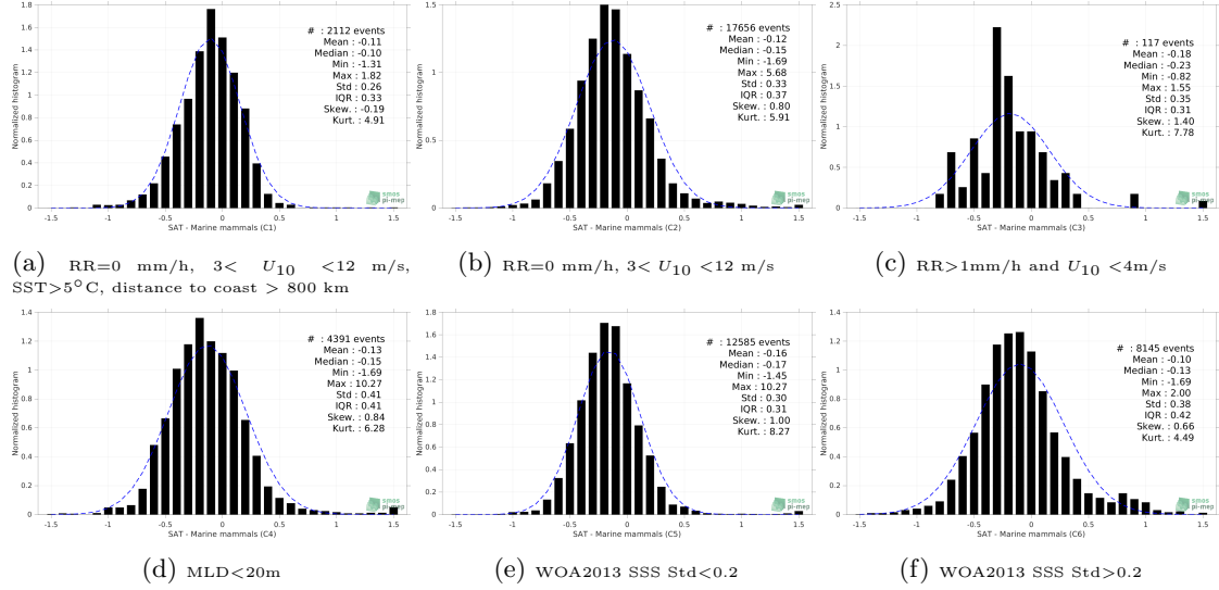
Figure 13: Normalized histogram of \Delta SSS (SMOS SSS L3 v7 - 18 Days (CATDS-CECOS-LOCEAN) - Marine mammals) for 6 different subdatasets corresponding to: RR=0 mm/h, 3 < U_{10} < 12 m/s, SST > 5°C, distance to coast > 800 km (a), RR=0 mm/h, 3 < U_{10} < 12 m/s (b), RR > 1mm/h and U_{10} < 4 m/s (c), MLD < 20m (d), WOA2013 SSS Std < 0.2 (e), WOA2013 SSS Std > 0.2 (f).
