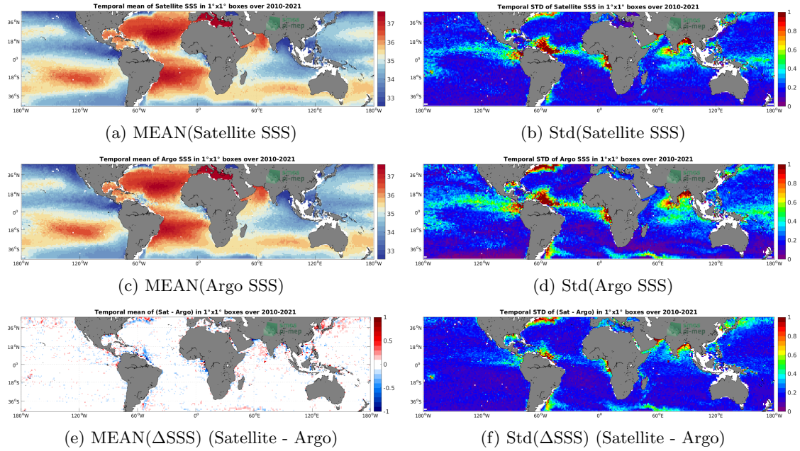
Figure 6: Temporal mean (left) and Std (right) of SSS from SMOS SSS L3 v7 - 18 Days (CATDS-CECOS-LOCEAN) (top), Argo (middle), and of \Delta SSS (Satellite - Argo). Only match-up pairs are used to generate these maps.
