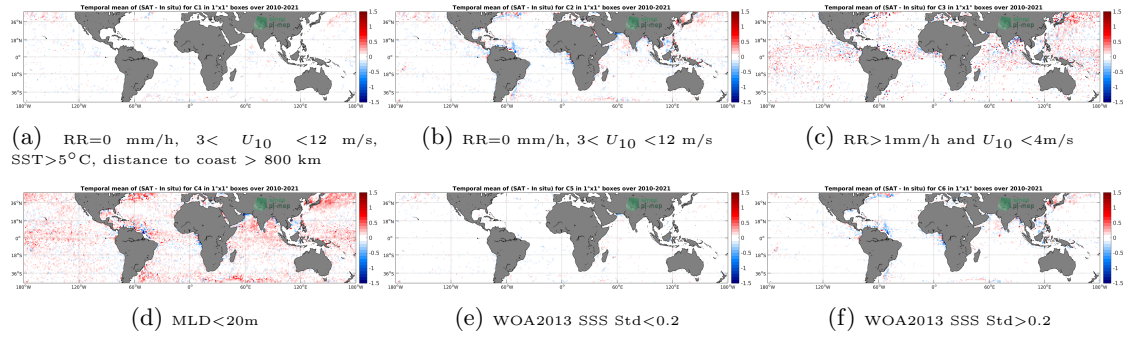
Figure 12: Temporal mean gridded over spatial boxes of size 1^\circ \times 1^\circ of \Delta SSS (SMOS SSS L3 v7 - 18 Days (CATDS-CECOS-LOCEAN) - Argo) for 6 different subdatasets corresponding to: RR=0 mm/h, 3 < U_{10} < 12 m/s, SST > 5^\circ C , distance to coast > 800 km (a), RR=0 mm/h, 3 < U_{10} < 12 m/s (b), RR > 1 mm/h and U_{10} < 4 m/s (c), MLD < 20 m (d), WOA2013 SSS Std < 0.2 (e), WOA2013 SSS Std > 0.2 (f).
