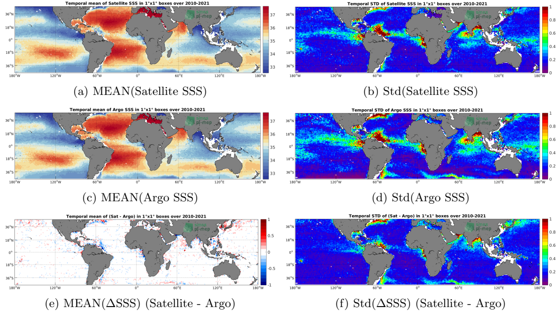
Figure 6: Temporal mean (left) and Std (right) of SSS from SMOS SSS L3 v7 - 18 Days (CATDS-CECOS-LOCEAN) (top), Argo (middle), and of \Delta SSS (Satellite - Argo). Only match-up pairs are used to generate these maps.
