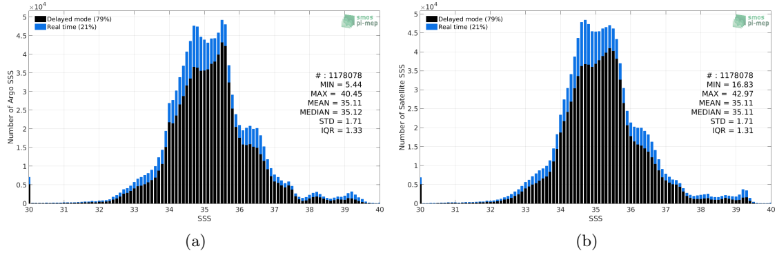
Figure 2: Histograms of SSS from Argo (a) and SMOS SSS L3 v7 - 18 Days (CATDS-CECOS-LOCEAN) (b) considering all match-up pairs per bins of 0.1 over the Mid-Low Latitudes 45N-45S Pi-MEP region and for the full satellite product period.
