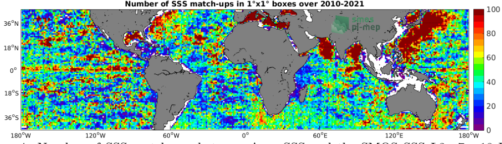
Figure 4: Number of SSS match-ups between Argo SSS and the SMOS SSS L3 v7 - 18 Days (CATDS-CECOS-LOCEAN) SSS product for the Mid-Low Latitudes 45N-45S Pi-MEP region over 1^\circ \times 1^\circ boxes and for the full satellite product period.
