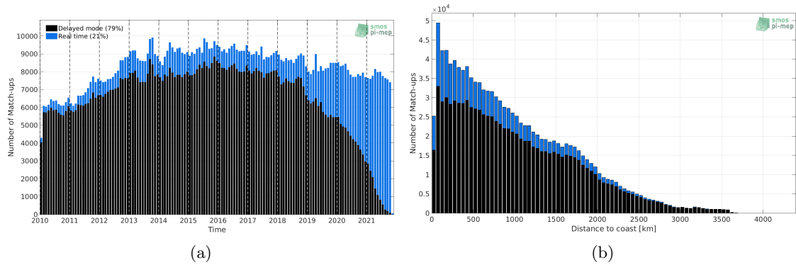
Figure 1: Number of match-ups between Argo and SMOS SSS L3 v7 - 18 Days (CATDS-CECOS-LOCEAN) SSS as a function of time (a) and as function of the distance to coast (b) over the Mid-Low Latitudes 45N-45S Pi-MEP region and for the full satellite product period.
