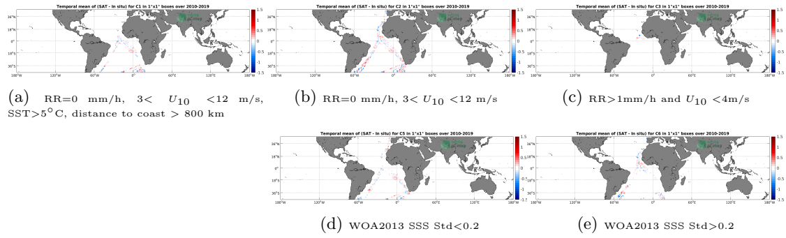
Figure 12: Temporal mean gridded over spatial boxes of size 1^\circ \times 1^\circ of \Delta SSS (SMOS SSS L3 v5 - 9 Days (CATDS-CECOS-LOCEAN) - TSG (Polarstern)) for 5 different subdatasets corresponding to: RR=0 mm/h, 3 < U_{10} < 12 m/s, SST > 5^\circ C , distance to coast > 800 km (a), RR=0 mm/h, 3 < U_{10} < 12 m/s (b), RR > 1 mm/h and U_{10} < 4 m/s (c), WOA2013 SSS Std < 0.2 (d), WOA2013 SSS Std > 0.2 (e).
