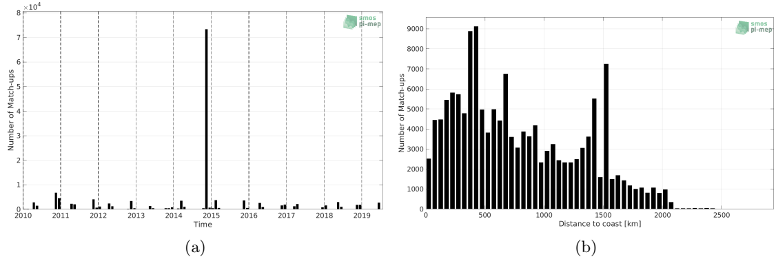
Figure 1: Number of match-ups between TSG (Polarstern) and SMOS SSS L3 v5 - 9 Days (CATDS-CECOS-LOCEAN) SSS as a function of time (a) and as function of the distance to coast (b) over the Mid-Low Latitudes 45N-45S Pi-MEP region and for the full satellite product period.
