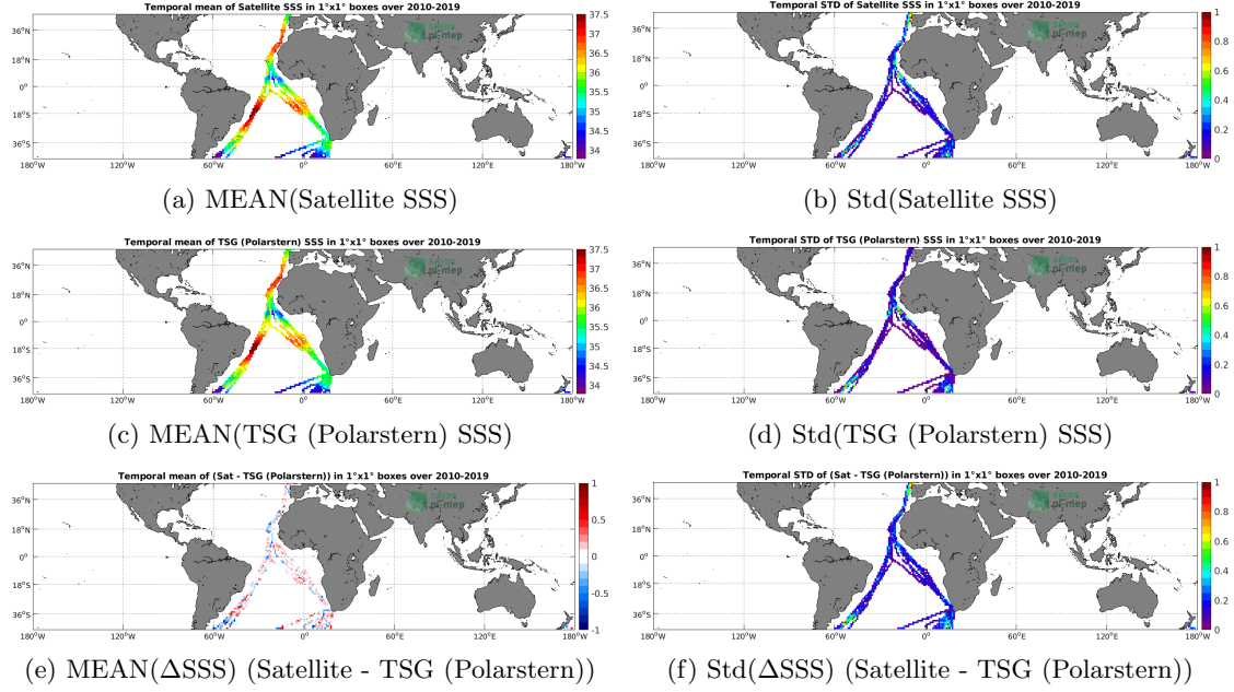
Figure 6: Temporal mean (left) and Std (right) of SSS from SMOS SSS L3 v5 - 9 Days (CATDS-CECOS-LOCEAN) (top), TSG (Polarstern) (middle), and of \Delta SSS (Satellite - TSG (Polarstern)). Only match-up pairs are used to generate these maps.
