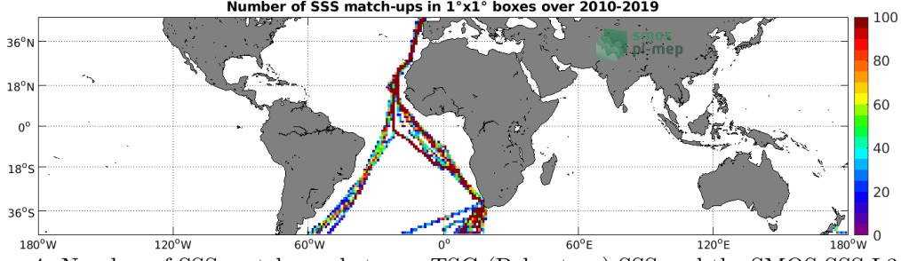
Figure 4: Number of SSS match-ups between TSG (Polarstern) SSS and the SMOS SSS L3 v5 - 9 Days (CATDS-CECOS-LOCEAN) SSS product for the Mid-Low Latitudes 45N-45S Pi-MEP region over 1^\circ \times 1^\circ boxes and for the full satellite product period.
