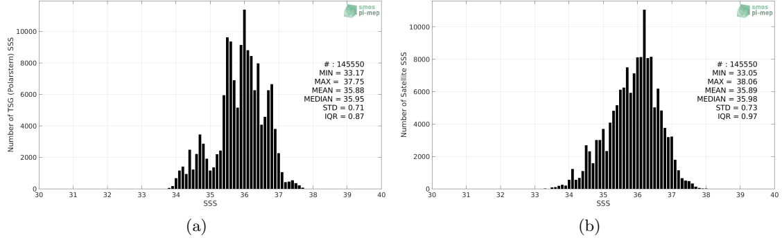
Figure 2: Histograms of SSS from TSG (Polarstern) (a) and SMOS SSS L3 v5 - 9 Days (CATDS-CECOS-LOCEAN) (b) considering all match-up pairs per bins of 0.1 over the Mid-Low Latitudes 45N-45S Pi-MEP region and for the full satellite product period.
