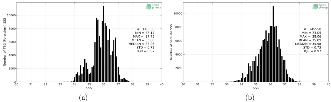
Figure 2: Histograms of SSS from TSG (Polarstern) (a) and SMOS SSS L3 v5 - 9 Days (CATDS-CECOS-LOCEAN) (b) considering all match-up pairs per bins of 0.1 over the Mid-Low Latitudes 45N-45S Pi-MEP region and for the full satellite product period.
