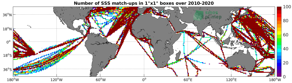
Figure 4: Number of SSS match-ups between TSG (LEGOS-DM) SSS and the SMOS SSS L3 v5 - 9 Days (CATDS-CECOS-LOCEAN) SSS product for the Mid-Low Latitudes 45N-45S Pi-MEP region over 1^\circ \times 1^\circ boxes and for the full satellite product period.
