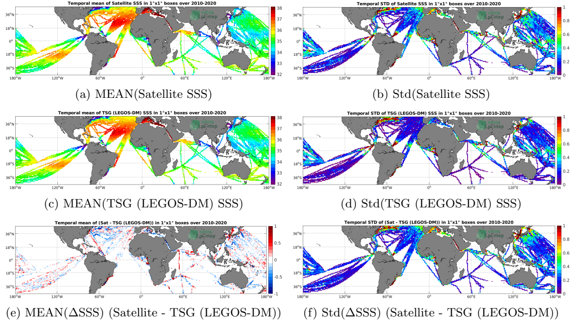
Figure 6: Temporal mean (left) and Std (right) of SSS from SMOS SSS L3 v5 - 9 Days (CATDS-CECOS-LOCEAN) (top), TSG (LEGOS-DM) (middle), and of \Delta SSS (Satellite - TSG (LEGOS-DM)). Only match-up pairs are used to generate these maps.
