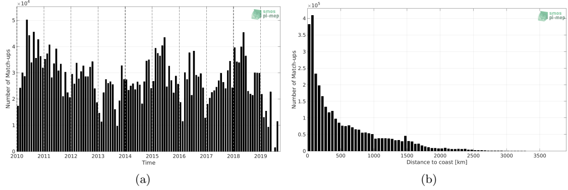
Figure 1: Number of match-ups between TSG (LEGOS-DM) and SMOS SSS L3 v5 - 9 Days (CATDS-CECOS-LOCEAN) SSS as a function of time (a) and as function of the distance to coast (b) over the Mid-Low Latitudes 45N-45S Pi-MEP region and for the full satellite product period.
