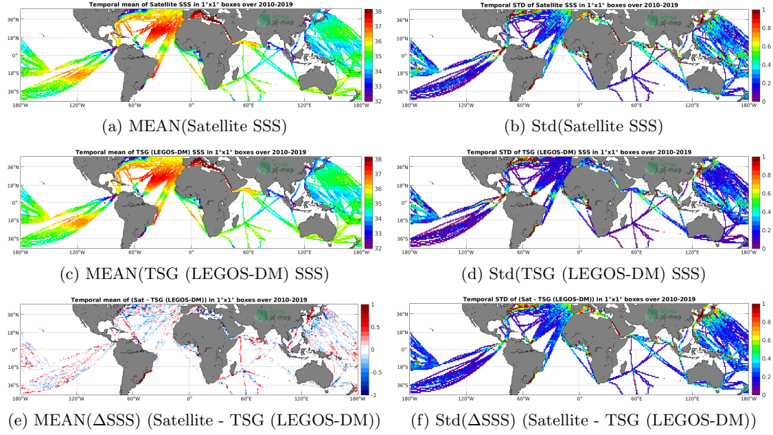
Figure 6: Temporal mean (left) and Std (right) of SSS from SMOS SSS L3 v5 - 9 Days (CATDS-CECOS-LOCEAN) (top), TSG (LEGOS-DM) (middle), and of \Delta SSS (Satellite - TSG (LEGOS-DM)). Only match-up pairs are used to generate these maps.
