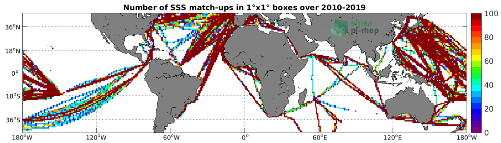
Figure 4: Number of SSS match-ups between TSG (LEGOS-DM) SSS and the SMOS SSS L3 v5 - 9 Days (CATDS-CECOS-LOCEAN) SSS product for the Mid-Low Latitudes 45N-45S Pi-MEP region over 1°x1° boxes and for the full satellite product period.
