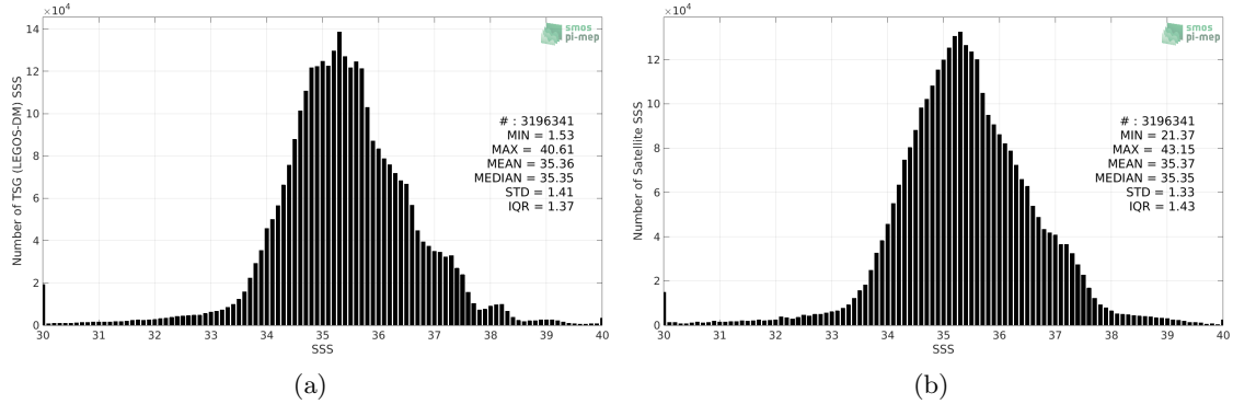
Figure 2: Histograms of SSS from TSG (LEGOS-DM) (a) and SMOS SSS L3 v5 - 9 Days (CATDS-CECOS-LOCEAN) (b) considering all match-up pairs per bins of 0.1 over the Mid-Low Latitudes 45N-45S Pi-MEP region and for the full satellite product period.
