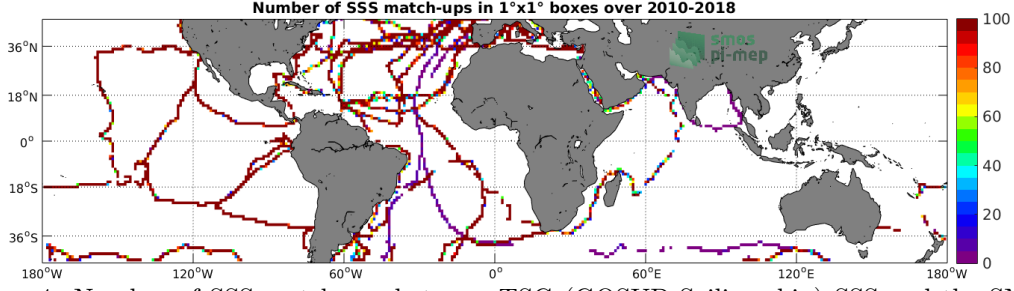
Figure 4: Number of SSS match-ups between TSG (GOSUD-Sailing-ship) SSS and the SMOS SSS L3 v5 - 9 Days (CATDS-CECOS-LOCEAN) SSS product for the Mid-Low Latitudes 45N-45S Pi-MEP region over 1^\circ \times 1^\circ boxes and for the full satellite product period.
