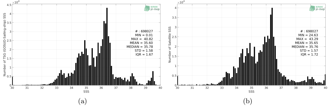
Figure 2: Histograms of SSS from TSG (GOSUD-Sailing-ship) (a) and SMOS SSS L3 v5 - 9 Days (CATDS-CECOS-LOCEAN) (b) considering all match-up pairs per bins of 0.1 over the Mid-Low Latitudes 45N-45S Pi-MEP region and for the full satellite product period.
