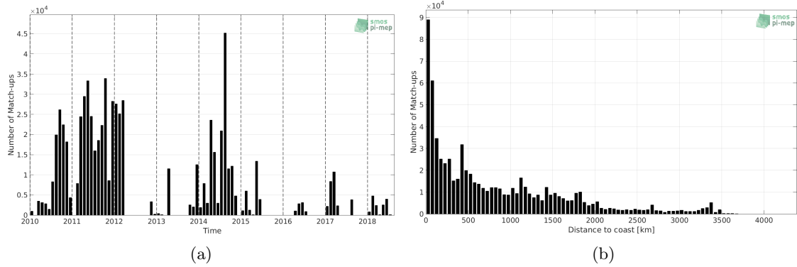
Figure 1: Number of match-ups between TSG (GOSUD-Sailing-ship) and SMOS SSS L3 v5 - 9 Days (CATDS-CECOS-LOCEAN) SSS as a function of time (a) and as function of the distance to coast (b) over the Mid-Low Latitudes 45N-45S Pi-MEP region and for the full satellite product period.
