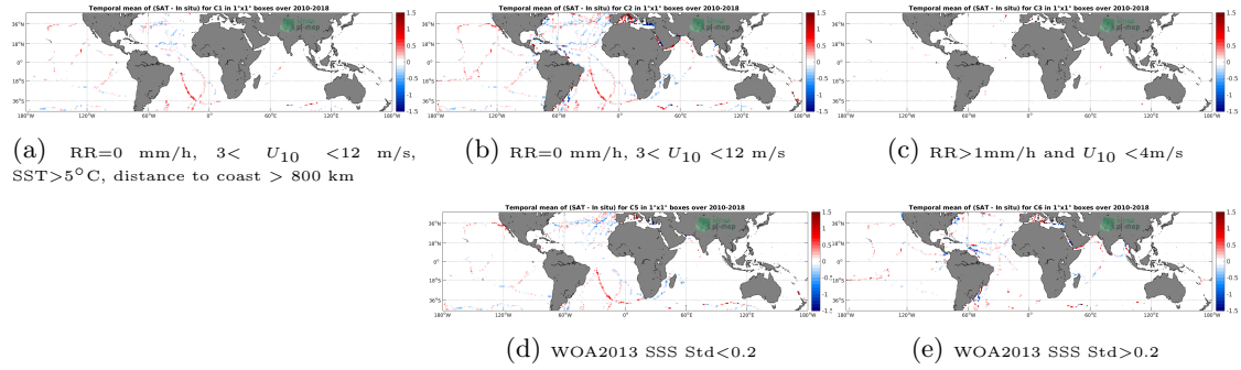
Figure 12: Temporal mean gridded over spatial boxes of size 1^\circ \times 1^\circ of \Delta SSS (SMOS SSS L3 v5 - 9 Days (CATDS-CECOS-LOCEAN) - TSG (GOSUD-Sailing-ship)) for 5 different subdatasets corresponding to: RR=0 mm/h, 3 < U_{10} < 12 m/s, SST > 5^\circ C , distance to coast > 800 km (a), RR=0 mm/h, 3 < U_{10} < 12 m/s (b), RR > 1 mm/h and U_{10} < 4 m/s (c), WOA2013 SSS Std < 0.2 (d), WOA2013 SSS Std > 0.2 (e).
