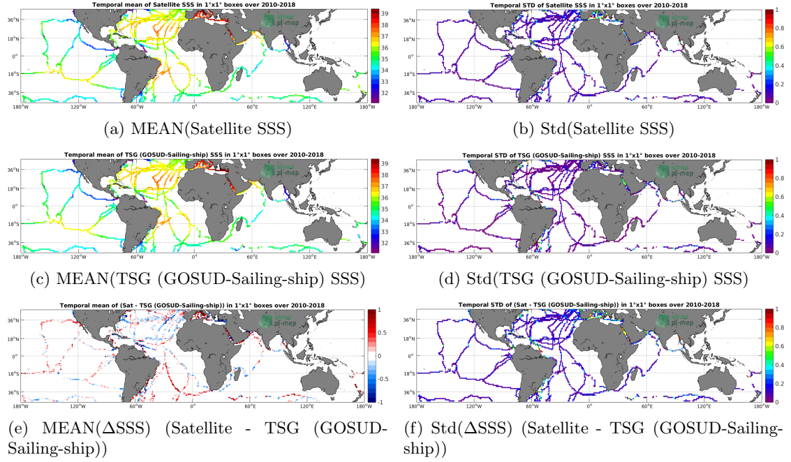
Figure 6: Temporal mean (left) and Std (right) of SSS from SMOS SSS L3 v5 - 9 Days (CATDS-CECOS-LOCEAN) (top), TSG (GOSUD-Sailing-ship) (middle), and of \Delta SSS (Satellite - TSG (GOSUD-Sailing-ship)). Only match-up pairs are used to generate these maps.
