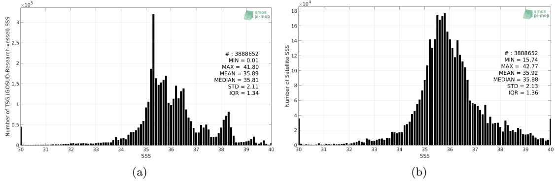
Figure 2: Histograms of SSS from TSG (GOSUD-Research-vessel) (a) and SMOS SSS L3 v5 - 9 Days (CATDS-CECOS-LOCEAN) (b) considering all match-up pairs per bins of 0.1 over the Mid-Low Latitudes 45N-45S Pi-MEP region and for the full satellite product period.
