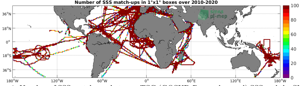
Figure 4: Number of SSS match-ups between TSG (GOSUD-Research-vessel) SSS and the SMOS SSS L3 v5 - 9 Days (CATDS-CECOS-LOCEAN) SSS product for the Mid-Low Latitudes 45N-45S Pi-MEP region over 1^\circ \times 1^\circ boxes and for the full satellite product period.
