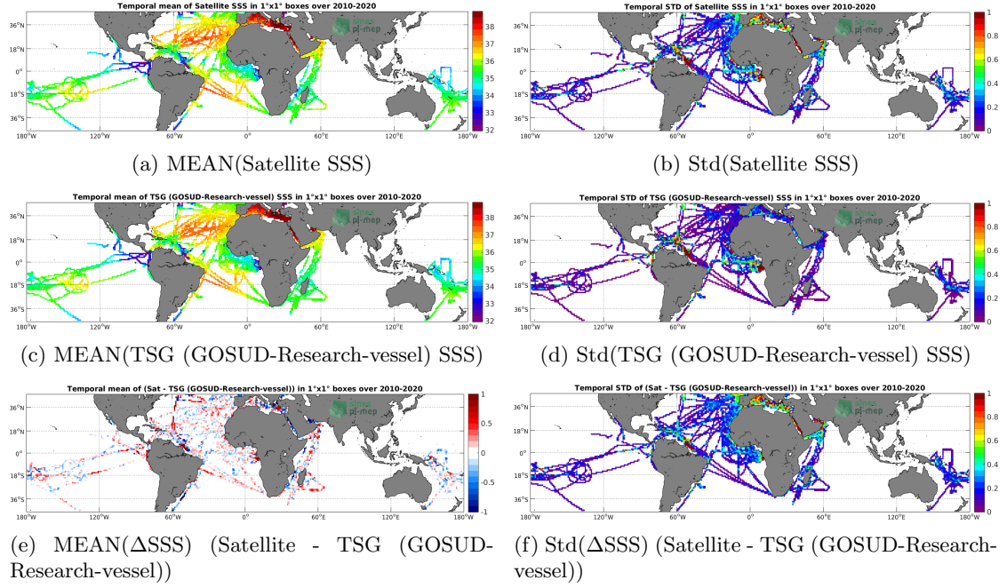
Figure 6: Temporal mean (left) and Std (right) of SSS from SMOS SSS L3 v5 - 9 Days (CATDS-CECOS-LOCEAN) (top), TSG (GOSUD-Research-vessel) (middle), and of \Delta SSS (Satellite - TSG (GOSUD-Research-vessel)). Only match-up pairs are used to generate these maps.
