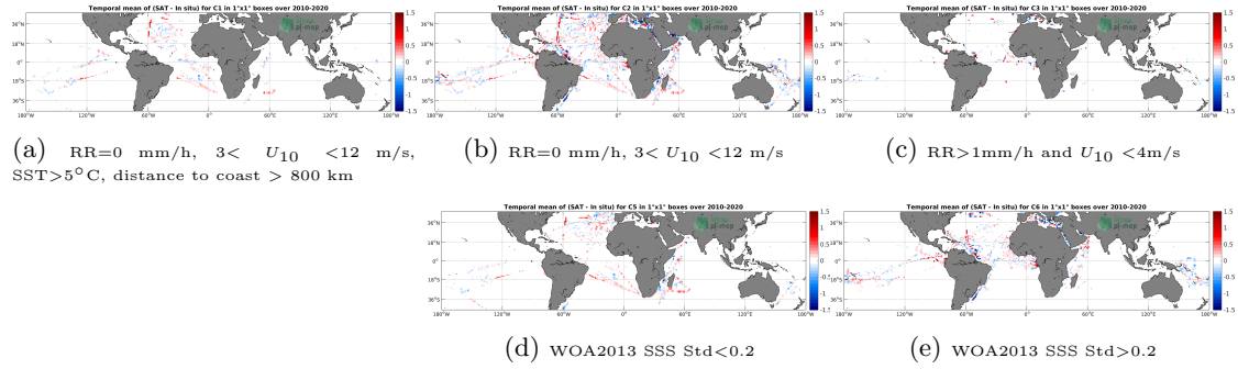
Figure 12: Temporal mean gridded over spatial boxes of size 1^\circ \times 1^\circ of \Delta SSS (SMOS SSS L3 v5 - 9 Days (CATDS-CECOS-LOCEAN) - TSG (GOSUD-Research-vessel)) for 5 different subdatasets corresponding to: RR=0 mm/h, 3 < U_{10} < 12 m/s, SST > 5^\circ C , distance to coast > 800 km (a), RR=0 mm/h, 3 < U_{10} < 12 m/s (b), RR > 1 mm/h and U_{10} < 4 m/s (c), WOA2013 SSS Std < 0.2 (d), WOA2013 SSS Std > 0.2 (e).
