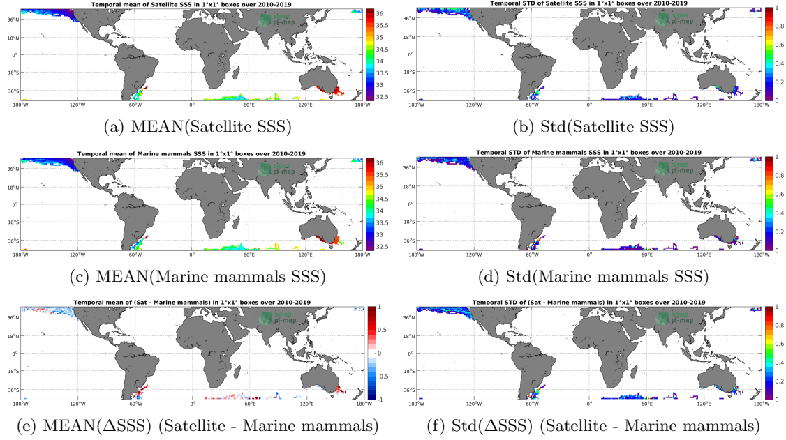
Figure 6: Temporal mean (left) and Std (right) of SSS from SMOS SSS L3 v5 - 9 Days (CATDS-CECOS-LOCEAN) (top), Marine mammals (middle), and of \Delta SSS (Satellite - Marine mammals). Only match-up pairs are used to generate these maps.
