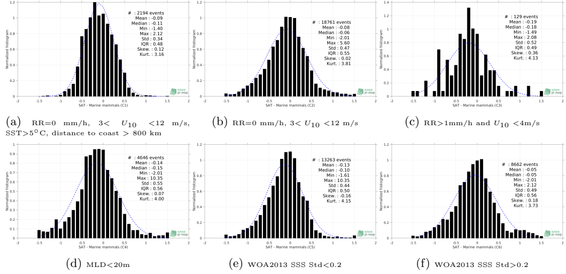
Figure 13: Normalized histogram of \Delta SSS (SMOS SSS L3 v5 - 9 Days (CATDS-CECOS-LOCEAN) - Marine mammals) for 6 different subdatasets corresponding to: RR=0 mm/h, 3 < U_{10} < 12 m/s, SST>5°C, distance to coast > 800 km (a), RR=0 mm/h, 3 < U_{10} < 12 m/s (b), RR>1mm/h and U_{10} < 4 m/s (c), MLD<20m (d), WOA2013 SSS Std<0.2 (e), WOA2013 SSS Std>0.2 (f).
