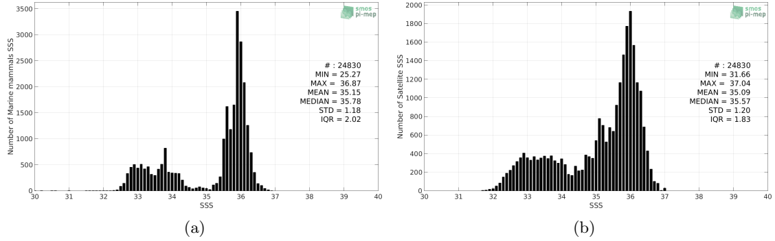
Figure 2: Histograms of SSS from Marine mammals (a) and SMOS SSS L3 v5 - 9 Days (CATDS-CECOS-LOCEAN) (b) considering all match-up pairs per bins of 0.1 over the Mid-Low Latitudes 45N-45S Pi-MEP region and for the full satellite product period.
