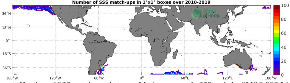
Figure 4: Number of SSS match-ups between Marine mammals SSS and the SMOS SSS L3 v5 - 9 Days (CATDS-CECOS-LOCEAN) SSS product for the Mid-Low Latitudes 45N-45S Pi-MEP region over 1^\circ \times 1^\circ boxes and for the full satellite product period.
