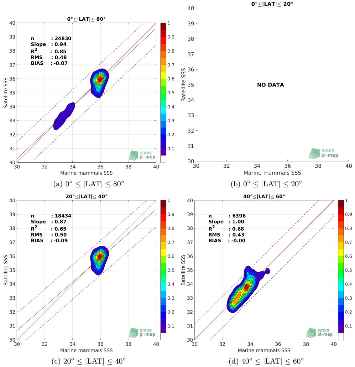
Figure 9: Contour maps of the concentration of SMOS SSS L3 v5 - 9 Days (CATDS-CECOS-LOCEAN) SSS (y-axis) versus Marine mammals SSS (x-axis) at match-up pairs for different latitude bands. For each plot, the red line shows x=y . The black thin and dashed lines indicate a linear fit through the data cloud and the \pm 95\% confidence levels, respectively. The number match-up pairs n , the slope and R^2 coefficient of the linear fit, the root mean square (RMS) and the mean bias between satellite and in situ data are indicated for each latitude band in each plots.
