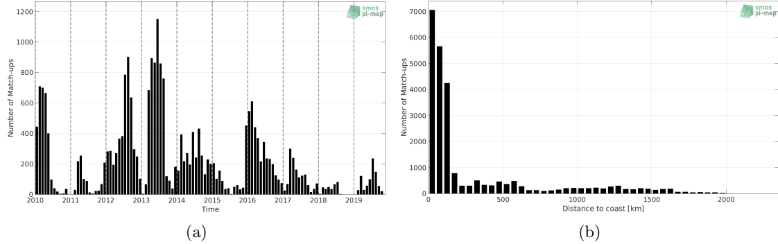
Figure 1: Number of match-ups between Marine mammals and SMOS SSS L3 v5 - 9 Days (CATDS-CECOS-LOCEAN) SSS as a function of time (a) and as function of the distance to coast (b) over the Mid-Low Latitudes 45N-45S Pi-MEP region and for the full satellite product period.
