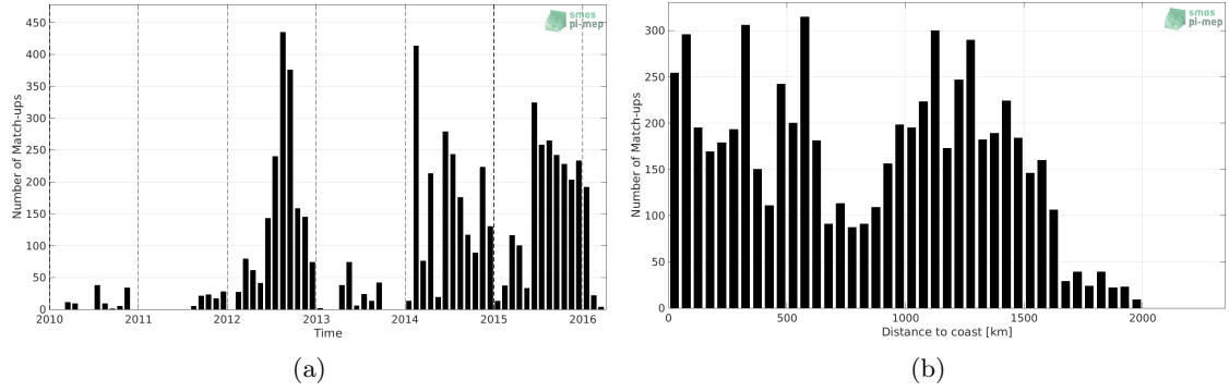
Figure 1: Number of match-ups between Sea mammals and SMOS SSS L3 v5 - 9 Days (CATDS-CECOS-LOCEAN) SSS as a function of time (a) and as function of the distance to coast (b) over the Mid-Low Latitudes 45N-45S Pi-MEP region and for the full satellite product period.
