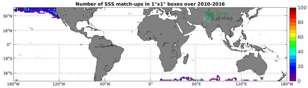
Figure 4: Number of SSS match-ups between Sea mammals SSS and the SMOS SSS L3 v5 - 9 Days (CATDS-CECOS-LOCEAN) SSS product for the Mid-Low Latitudes 45N-45S Pi-MEP region over 1°x1° boxes and for the full satellite product period.
