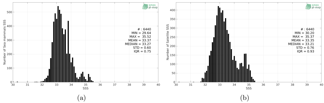
Figure 2: Histograms of SSS from Sea mammals (a) and SMOS SSS L3 v5 - 9 Days (CATDS-CECOS-LOCEAN) (b) considering all match-up pairs per bins of 0.1 over the Mid-Low Latitudes 45N-45S Pi-MEP region and for the full satellite product period.
