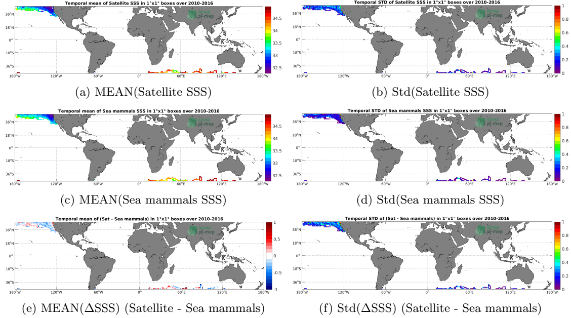
Figure 6: Temporal mean (left) and Std (right) of SSS from SMOS SSS L3 v5 - 9 Days (CATDS-CECOS-LOCEAN) (top), Sea mammals (middle), and of \Delta SSS (Satellite - Sea mammals). Only match-up pairs are used to generate these maps.
