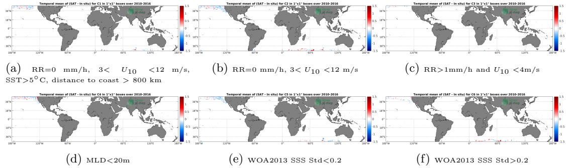
Figure 12: Temporal mean gridded over spatial boxes of size 1^\circ \times 1^\circ of \Delta SSS (SMOS SSS L3 v5 - 9 Days (CATDS-CECOS-LOCEAN) - Sea mammals) for 6 different subdatasets corresponding to: RR=0 mm/h, 3 < U_{10} < 12 m/s, SST > 5^\circ C , distance to coast > 800 km (a), RR=0 mm/h, 3 < U_{10} < 12 m/s (b), RR > 1 mm/h and U_{10} < 4 m/s (c), MLD < 20 m (d), WOA2013 SSS Std < 0.2 (e), WOA2013 SSS Std > 0.2 (f).
