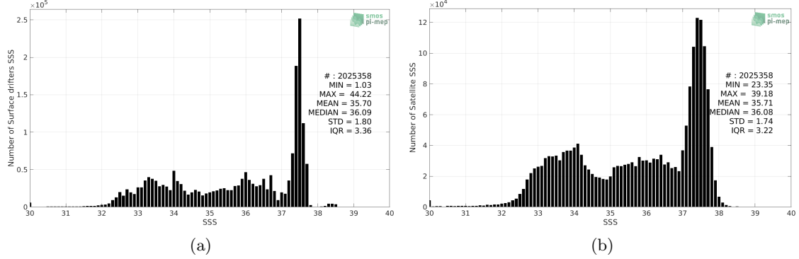
Figure 2: Histograms of SSS from Surface drifters (a) and SMOS SSS L3 v5 - 9 Days (CATDS-CECOS-LOCEAN) (b) considering all match-up pairs per bins of 0.1 over the Mid-Low Latitudes 45N-45S Pi-MEP region and for the full satellite product period.
