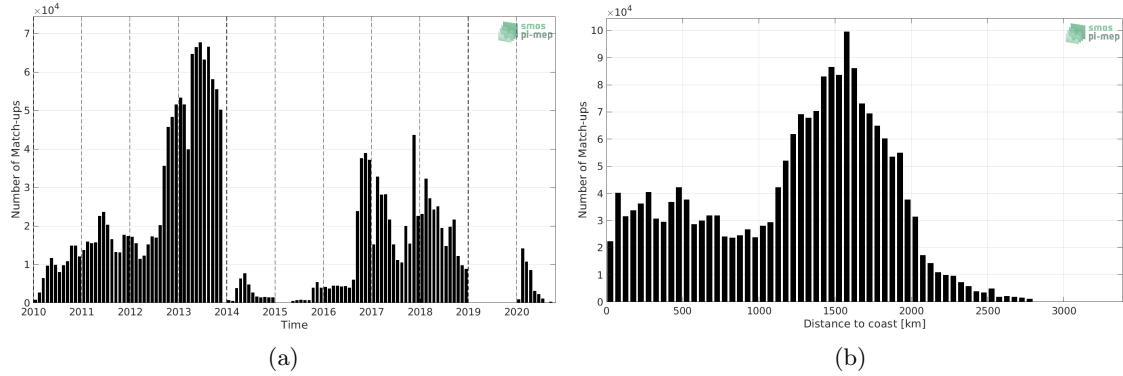
Figure 1: Number of match-ups between Surface drifters and SMOS SSS L3 v5 - 9 Days (CATDS-CECOS-LOCEAN) SSS as a function of time (a) and as function of the distance to coast (b) over the Mid-Low Latitudes 45N-45S Pi-MEP region and for the full satellite product period.
