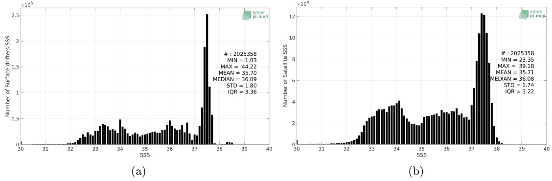
Figure 2: Histograms of SSS from Surface drifters (a) and SMOS SSS L3 v5 - 9 Days (CATDS-CECOS-LOCEAN) (b) considering all match-up pairs per bins of 0.1 over the Mid-Low Latitudes 45N-45S Pi-MEP region and for the full satellite product period.
