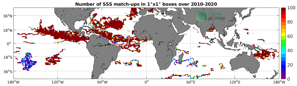
Figure 3: Number of SSS match-ups between Surface drifters SSS and the SMOS SSS L3 v5 - 9 Days (CATDS-CECOS-LOCEAN) SSS product for the Mid-Low Latitudes 45N-45S Pi-MEP region over 1^\circ \times 1^\circ boxes and for the full satellite product period.
