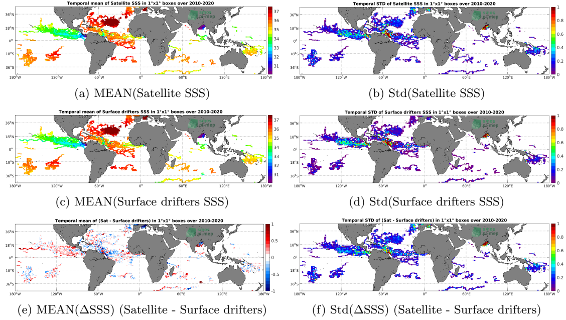
Figure 5: Temporal mean (left) and Std (right) of SSS from SMOS SSS L3 v5 - 9 Days (CATDS-CECOS-LOCEAN) (top), Surface drifters (middle), and of \Delta SSS (Satellite - Surface drifters). Only match-up pairs are used to generate these maps.
