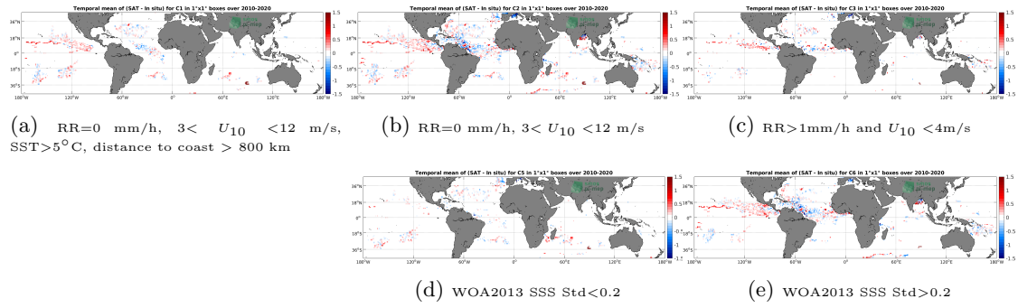
Figure 11: Temporal mean gridded over spatial boxes of size 1^\circ \times 1^\circ of \Delta SSS (SMOS SSS L3 v5 - 9 Days (CATDS-CECOS-LOCEAN) - Surface drifters) for 5 different subdatasets corresponding to: RR=0 mm/h, 3 < U_{10} < 12 m/s, SST >5^\circ\text{C} , distance to coast > 800 km (a), RR=0 mm/h, 3 < U_{10} < 12 m/s (b), RR >1 mm/h and U_{10} < 4 m/s (c), WOA2013 SSS Std <0.2 (d), WOA2013 SSS Std >0.2 (e).
