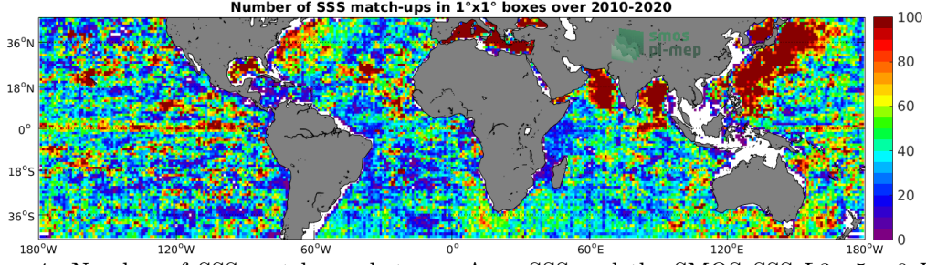
Figure 4: Number of SSS match-ups between Argo SSS and the SMOS SSS L3 v5 - 9 Days (CATDS-CECOS-LOCEAN) SSS product for the Mid-Low Latitudes 45N-45S Pi-MEP region over 1^\circ \times 1^\circ boxes and for the full satellite product period.
