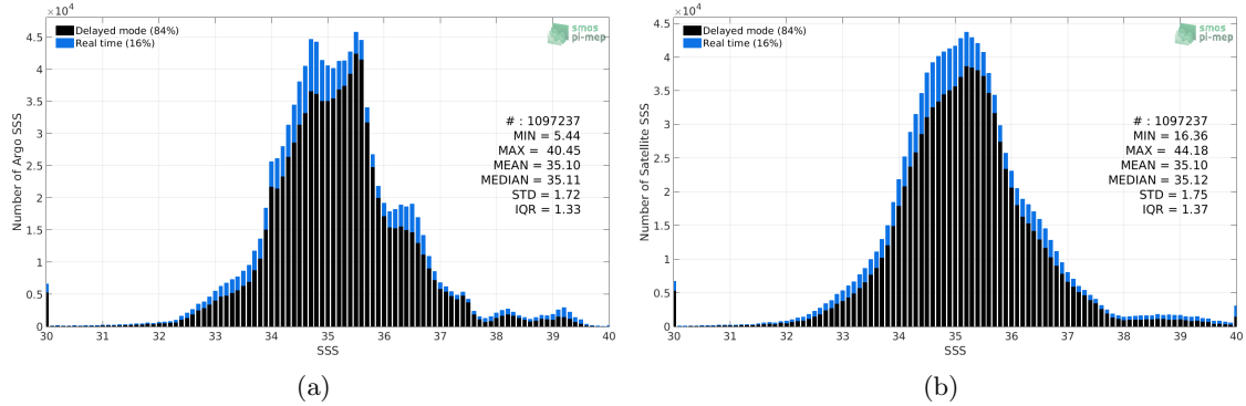
Figure 2: Histograms of SSS from Argo (a) and SMOS SSS L3 v5 - 9 Days (CATDS-CECOS-LOCEAN) (b) considering all match-up pairs per bins of 0.1 over the Mid-Low Latitudes 45N-45S Pi-MEP region and for the full satellite product period.
