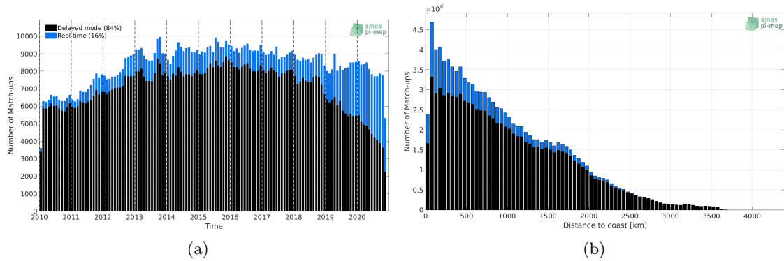
Figure 1: Number of match-ups between Argo and SMOS SSS L3 v5 - 9 Days (CATDS-CECOS-LOCEAN) SSS as a function of time (a) and as function of the distance to coast (b) over the Mid-Low Latitudes 45N-45S Pi-MEP region and for the full satellite product period.
