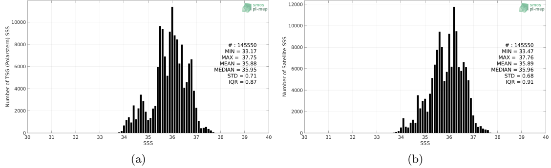
Figure 2: Histograms of SSS from TSG (Polarstern) (a) and SMOS SSS L3 v5 - 18 Days (CATDS-CECOS-LOCEAN) (b) considering all match-up pairs per bins of 0.1 over the Mid-Low Latitudes 45N-45S Pi-MEP region and for the full satellite product period.
