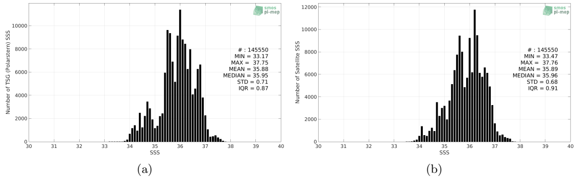
Figure 2: Histograms of SSS from TSG (Polarstern) (a) and SMOS SSS L3 v5 - 18 Days (CATDS-CECOS-LOCEAN) (b) considering all match-up pairs per bins of 0.1 over the Mid-Low Latitudes 45N-45S Pi-MEP region and for the full satellite product period.
