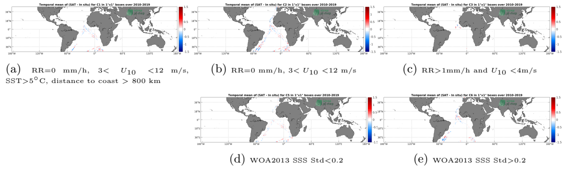
Figure 12: Temporal mean gridded over spatial boxes of size 1^\circ \times 1^\circ of \Delta SSS (SMOS SSS L3 v5 - 18 Days (CATDS-CECOS-LOCEAN) - TSG (Polarstern)) for 5 different subdatasets corresponding to: RR=0 mm/h, 3 < U_{10} < 12 m/s, SST > 5^\circ C , distance to coast > 800 km (a), RR=0 mm/h, 3 < U_{10} < 12 m/s (b), RR > 1 mm/h and U_{10} < 4 m/s (c), WOA2013 SSS Std < 0.2 (d), WOA2013 SSS Std > 0.2 (e).
