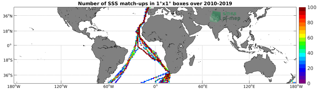
Figure 4: Number of SSS match-ups between TSG (Polarstern) SSS and the SMOS SSS L3 v5 - 18 Days (CATDS-CECOS-LOCEAN) SSS product for the Mid-Low Latitudes 45N-45S Pi-MEP region over 1^\circ \times 1^\circ boxes and for the full satellite product period.
