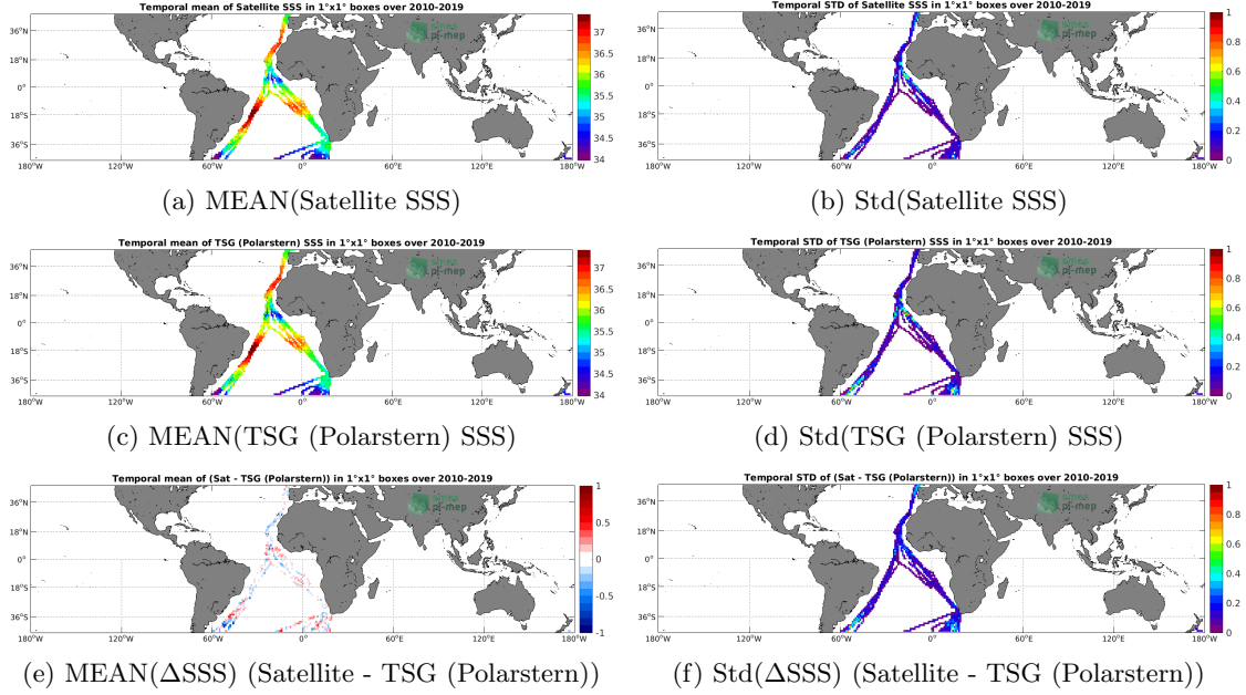
Figure 6: Temporal mean (left) and Std (right) of SSS from SMOS SSS L3 v5 - 18 Days (CATDS-CECOS-LOCEAN) (top), TSG (Polarstern) (middle), and of \Delta SSS (Satellite - TSG (Polarstern)). Only match-up pairs are used to generate these maps.
