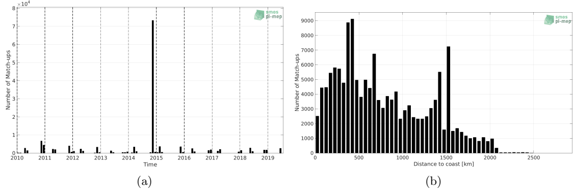
Figure 1: Number of match-ups between TSG (Polarstern) and SMOS SSS L3 v5 - 18 Days (CATDS-CECOS-LOCEAN) SSS as a function of time (a) and as function of the distance to coast (b) over the Mid-Low Latitudes 45N-45S Pi-MEP region and for the full satellite product period.
