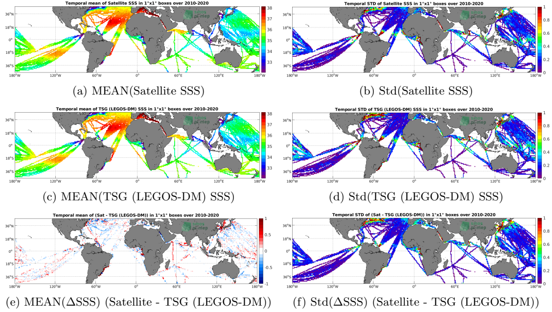
Figure 6: Temporal mean (left) and Std (right) of SSS from SMOS SSS L3 v5 - 18 Days (CATDS-CECOS-LOCEAN) (top), TSG (LEGOS-DM) (middle), and of \Delta SSS (Satellite - TSG (LEGOS-DM)). Only match-up pairs are used to generate these maps.
