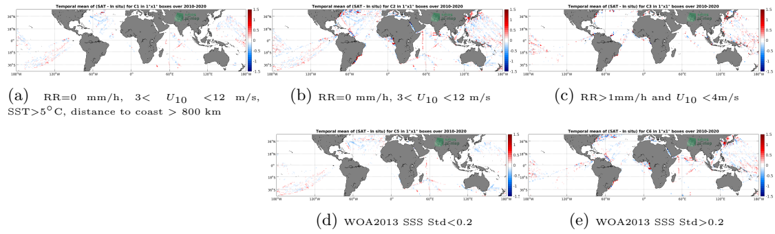
Figure 12: Temporal mean gridded over spatial boxes of size 1^\circ \times 1^\circ of \Delta SSS (SMOS SSS L3 v5 - 18 Days (CATDS-CECOS-LOCEAN) - TSG (LEGOS-DM)) for 5 different subdatasets corresponding to: RR=0 mm/h, 3 < U_{10} < 12 m/s, SST > 5^\circ C , distance to coast > 800 km (a), RR=0 mm/h, 3 < U_{10} < 12 m/s (b), RR > 1 mm/h and U_{10} < 4 m/s (c), WOA2013 SSS Std < 0.2 (d), WOA2013 SSS Std > 0.2 (e).
