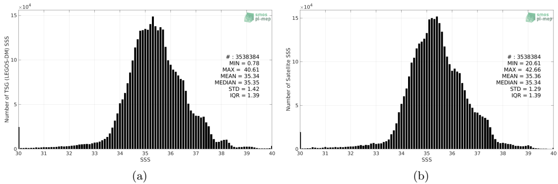
Figure 2: Histograms of SSS from TSG (LEGOS-DM) (a) and SMOS SSS L3 v5 - 18 Days (CATDS-CECOS-LOCEAN) (b) considering all match-up pairs per bins of 0.1 over the Mid-Low Latitudes 45N-45S Pi-MEP region and for the full satellite product period.
