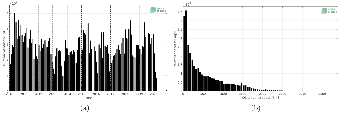
Figure 1: Number of match-ups between TSG (LEGOS-DM) and SMOS SSS L3 v5 - 18 Days (CATDS-CECOS-LOCEAN) SSS as a function of time (a) and as function of the distance to coast (b) over the Mid-Low Latitudes 45N-45S Pi-MEP region and for the full satellite product period.
