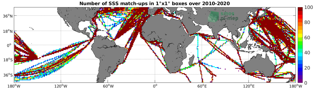
Figure 4: Number of SSS match-ups between TSG (LEGOS-DM) SSS and the SMOS SSS L3 v5 - 18 Days (CATDS-CECOS-LOCEAN) SSS product for the Mid-Low Latitudes 45N-45S Pi-MEP region over 1^\circ \times 1^\circ boxes and for the full satellite product period.
