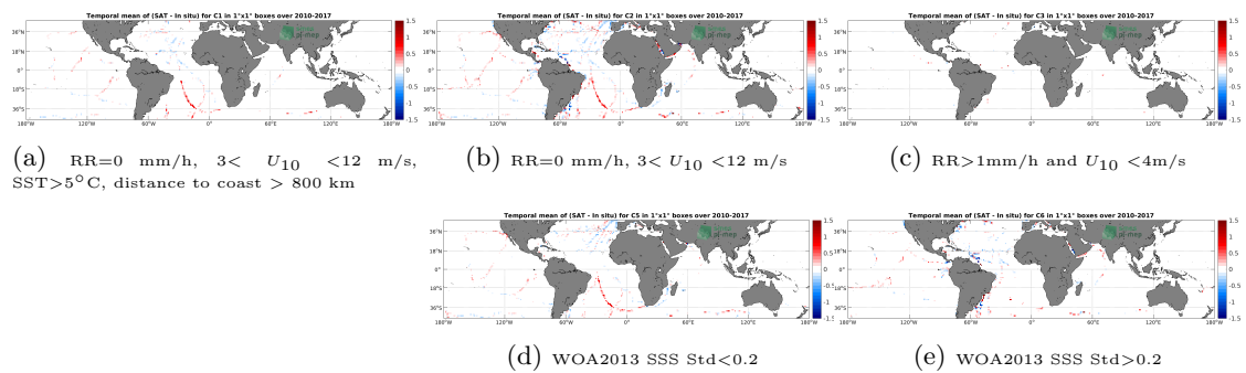
Figure 12: Temporal mean gridded over spatial boxes of size 1^\circ \times 1^\circ of \Delta\text{SSS} (SMOS SSS L3 v5 - 18 Days (CATDS-CECOS-LOCEAN) - TSG (GOSUD-Sailing-ship)) for 5 different subdatasets corresponding to:RR=0 mm/h, 3 < U_{10} < 12 m/s, SST>5°C, distance to coast > 800 km (a), RR=0 mm/h, 3 < U_{10} < 12 m/s (b), RR>1mm/h and U_{10} < 4 m/s (c), WOA2013 SSS Std<0.2 (d), WOA2013 SSS Std>0.2 (e).
