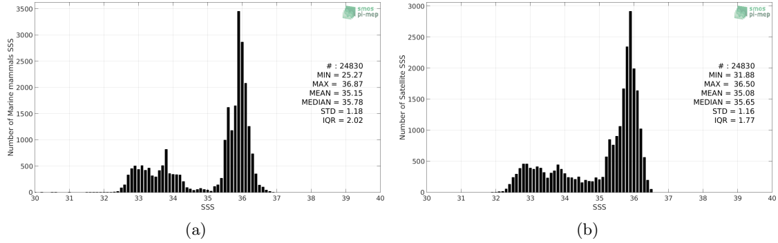
Figure 2: Histograms of SSS from Marine mammals (a) and SMOS SSS L3 v5 - 18 Days (CATDS-CECOS-LOCEAN) (b) considering all match-up pairs per bins of 0.1 over the Mid-Low Latitudes 45N-45S Pi-MEP region and for the full satellite product period.
