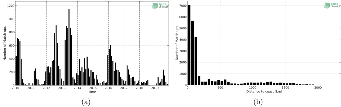
Figure 1: Number of match-ups between Marine mammals and SMOS SSS L3 v5 - 18 Days (CATDS-CECOS-LOCEAN) SSS as a function of time (a) and as function of the distance to coast (b) over the Mid-Low Latitudes 45N-45S Pi-MEP region and for the full satellite product period.
