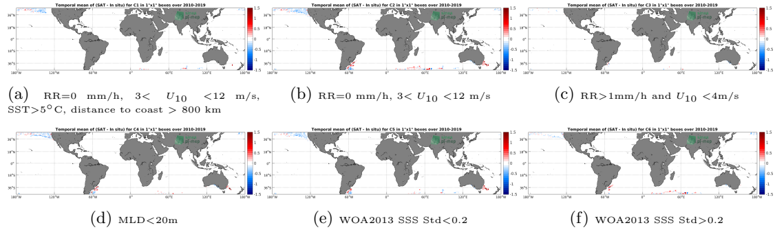
Figure 12: Temporal mean gridded over spatial boxes of size 1^{\circ} \times 1^{\circ} of \Delta\text{SSS} (SMOS SSS L3 v5 - 18 Days (CATDS-CECOS-LOCEAN) - Marine mammals) for 6 different subdatasets corresponding to: \text{RR}=0 mm/h, 3 < U_{10} < 12 m/s, \text{SST}>5^{\circ}\text{C} , distance to coast > 800 km (a), \text{RR}=0 mm/h, 3 < U_{10} < 12 m/s (b), \text{RR}>1\text{mm/h} and U_{10} < 4\text{m/s} (c), \text{MLD}<20\text{m} (d), \text{WOA2013 SSS Std}<0.2 (e), \text{WOA2013 SSS Std}>0.2 (f).
