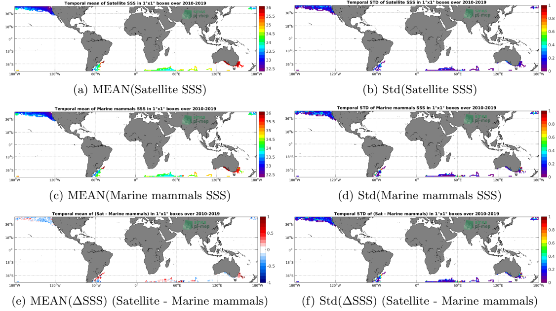
Figure 6: Temporal mean (left) and Std (right) of SSS from SMOS SSS L3 v5 - 18 Days (CATDS-CECOS-LOCEAN) (top), Marine mammals (middle), and of \Delta SSS (Satellite - Marine mammals). Only match-up pairs are used to generate these maps.
