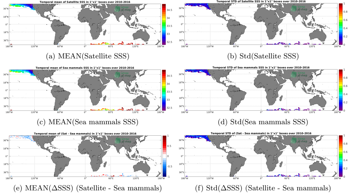
Figure 6: Temporal mean (left) and Std (right) of SSS from SMOS SSS L3 v5 - 18 Days (CATDS-CECOS-LOCEAN) (top), Sea mammals (middle), and of \Delta SSS (Satellite - Sea mammals). Only match-up pairs are used to generate these maps.
