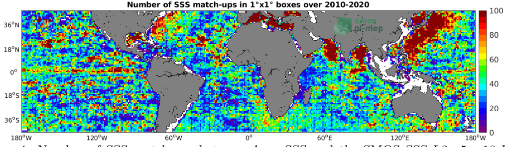
Figure 4: Number of SSS match-ups between Argo SSS and the SMOS SSS L3 v5 - 18 Days (CATDS-CECOS-LOCEAN) SSS product for the Mid-Low Latitudes 45N-45S Pi-MEP region over 1°x1° boxes and for the full satellite product period.
