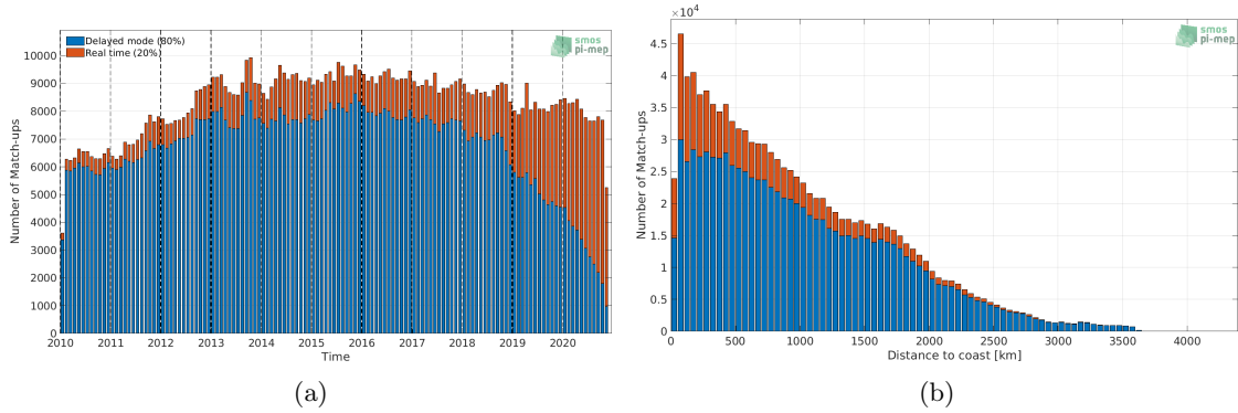
Figure 1: Number of match-ups between Argo and SMOS SSS L3 v5 - 18 Days (CATDS-CECOS-LOCEAN) SSS as a function of time (a) and as function of the distance to coast (b) over the Mid-Low Latitudes 45N-45S Pi-MEP region and for the full satellite product period.
