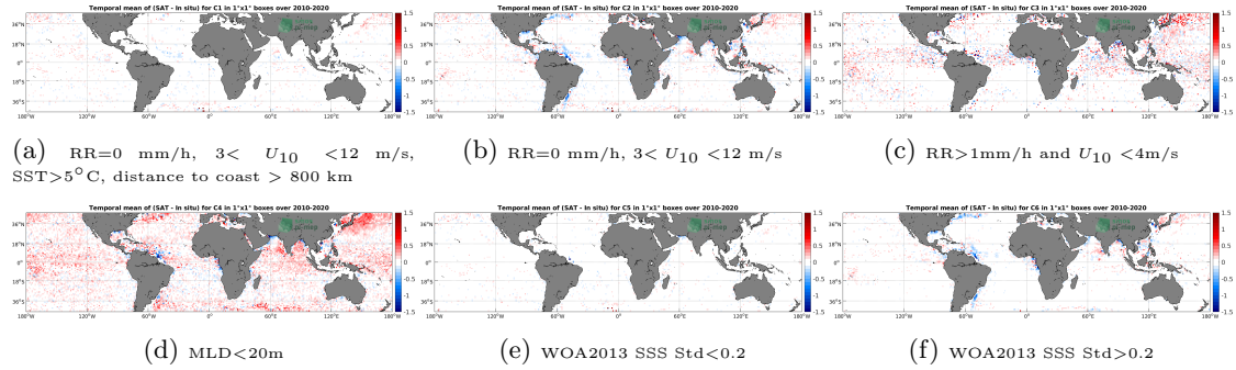
Figure 12: Temporal mean gridded over spatial boxes of size 1^\circ \times 1^\circ of \Delta SSS (SMOS SSS L3 v5 - 18 Days (CATDS-CECOS-LOCEAN) - Argo) for 6 different subdatasets corresponding to:RR=0 mm/h, 3 < U_{10} < 12 m/s, SST >5^\circ\text{C} , distance to coast > 800 km (a), RR=0 mm/h, 3 < U_{10} < 12 m/s (b), RR >1 mm/h and U_{10} < 4 m/s (c),MLD <20 m (d),WOA2013 SSS Std <0.2 (e),WOA2013 SSS Std >0.2 (f).
