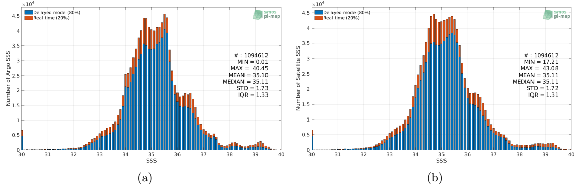
Figure 2: Histograms of SSS from Argo (a) and SMOS SSS L3 v5 - 18 Days (CATDS-CECOS-LOCEAN) (b) considering all match-up pairs per bins of 0.1 over the Mid-Low Latitudes 45N-45S Pi-MEP region and for the full satellite product period.
