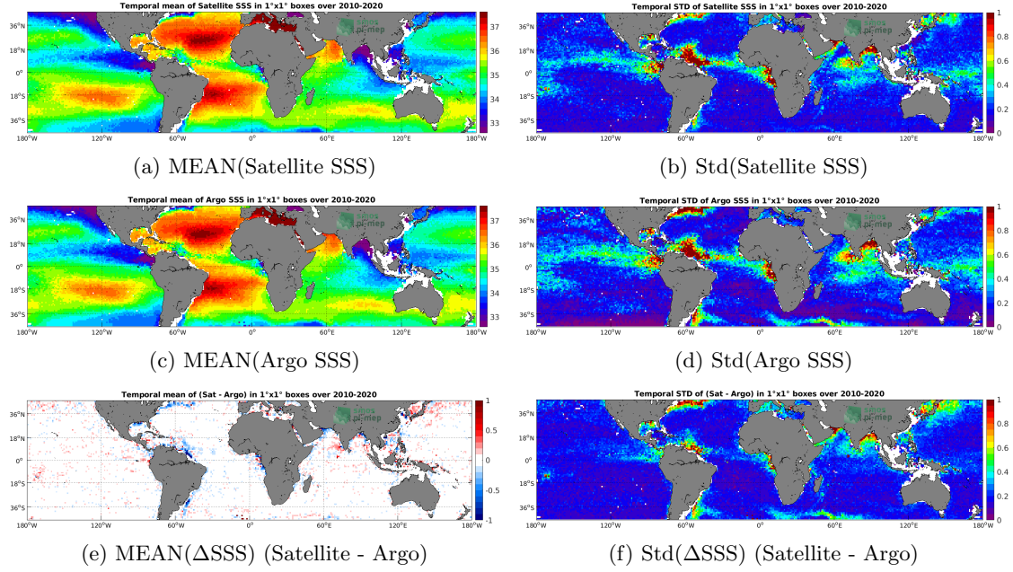
Figure 6: Temporal mean (left) and Std (right) of SSS from SMOS SSS L3 v5 - 18 Days (CATDS-CECOS-LOCEAN) (top), Argo (middle), and of \Delta SSS (Satellite - Argo). Only match-up pairs are used to generate these maps.
