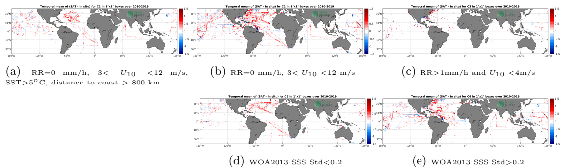
Figure 12: Temporal mean gridded over spatial boxes of size 1^\circ \times 1^\circ of \Delta SSS (SMOS SSS L3 v4 - 9 Days (CATDS-CECOS-LOCEAN) - TSG (SAMOS)) for 5 different subdatasets corresponding to:RR=0 mm/h, 3 < U_{10} < 12 m/s, SST >5^\circ\text{C} , distance to coast > 800 km (a), RR=0 mm/h, 3 < U_{10} < 12 m/s (b), RR >1 mm/h and U_{10} < 4 m/s (c), WOA2013 SSS Std <0.2 (d), WOA2013 SSS Std >0.2 (e).
