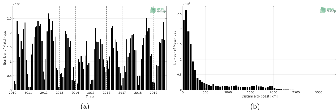
Figure 1: Number of match-ups between TSG (SAMOS) and SMOS SSS L3 v4 - 9 Days (CATDS-CECOS-LOCEAN) SSS as a function of time (a) and as function of the distance to coast (b) over the Mid-Low Latitudes 45N-45S Pi-MEP region and for the full satellite product period.
