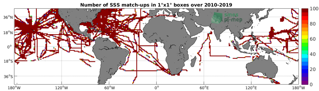
Figure 4: Number of SSS match-ups between TSG (SAMOS) SSS and the SMOS SSS L3 v4 - 9 Days (CATDS-CECOS-LOCEAN) SSS product for the Mid-Low Latitudes 45N-45S Pi-MEP region over 1°x1° boxes and for the full satellite product period.
