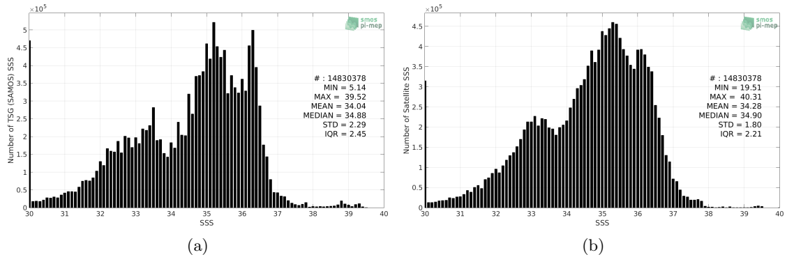
Figure 2: Histograms of SSS from TSG (SAMOS) (a) and SMOS SSS L3 v4 - 9 Days (CATDS-CECOS-LOCEAN) (b) considering all match-up pairs per bins of 0.1 over the Mid-Low Latitudes 45N-45S Pi-MEP region and for the full satellite product period.
