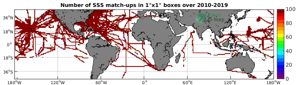
Figure 4: Number of SSS match-ups between TSG-SAMOS SSS and the SMOS-L3-CATDS-CECOS-LOCEAN-V4-9DAYS-25KM SSS product for the Mid-Low Latitudes 45N-45S Pi-MEP region over 1°x1° boxes and for the full satellite product period.
