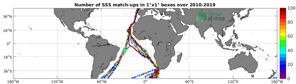
Figure 4: Number of SSS match-ups between TSG-POLARSTERN SSS and the SMOS-L3-CATDS-CECOS-LOCEAN-V4-9DAYS-25KM SSS product for the Mid-Low Latitudes 45N-45S Pi-MEP region over 1^\circ \times 1^\circ boxes and for the full satellite product period.
