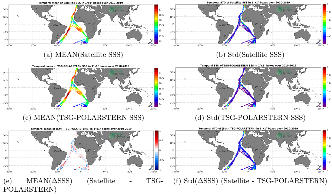
Figure 6: Temporal mean (left) and Std (right) of SSS from SMOS-L3-CATDS-CECOS-LOCEAN-V4-9DAYS-25KM (top), TSG-POLARSTERN (middle), and of \Delta SSS (Satellite - TSG-POLARSTERN). Only match-up pairs are used to generate these maps.
