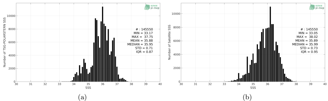
Figure 2: Histograms of SSS from TSG-POLARSTERN (a) and SMOS-L3-CATDS-CECOS-LOCEAN-V4-9DAYS-25KM (b) considering all match-up pairs per bins of 0.1 over the Mid-Low Latitudes 45N-45S Pi-MEP region and for the full satellite product period.
