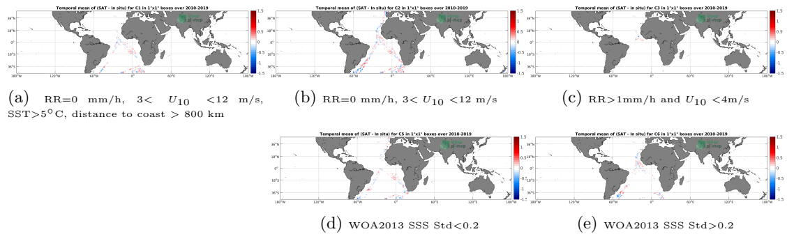
Figure 12: Temporal mean gridded over spatial boxes of size 1^\circ \times 1^\circ of \Delta SSS (SMOS-L3-CATDS-CECOS-LOCEAN-V4-9DAYS-25KM - TSG-POLARSTERN) for 5 different subdatasets corresponding to:RR=0 mm/h, 3 < U_{10} < 12 m/s, SST >5^\circ C, distance to coast > 800 km (a), RR=0 mm/h, 3 < U_{10} < 12 m/s (b), RR >1 mm/h and U_{10} < 4 m/s (c), WOA2013 SSS Std <0.2 (d), WOA2013 SSS Std >0.2 (e).
