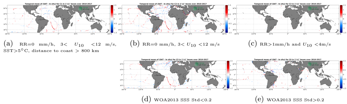
Figure 12: Temporal mean gridded over spatial boxes of size 1^\circ \times 1^\circ of \Delta\text{SSS} (SMOS SSS L3 v4 - 9 Days (CATDS-CECOS-LOCEAN) - TSG (GOSUD-Sailing-ship)) for 5 different subdatasets corresponding to: RR=0 mm/h, 3 < U_{10} < 12 m/s, SST > 5°C, distance to coast > 800 km (a), RR=0 mm/h, 3 < U_{10} < 12 m/s (b), RR > 1mm/h and U_{10} < 4 m/s (c), WOA2013 SSS Std < 0.2 (d), WOA2013 SSS Std > 0.2 (e).
