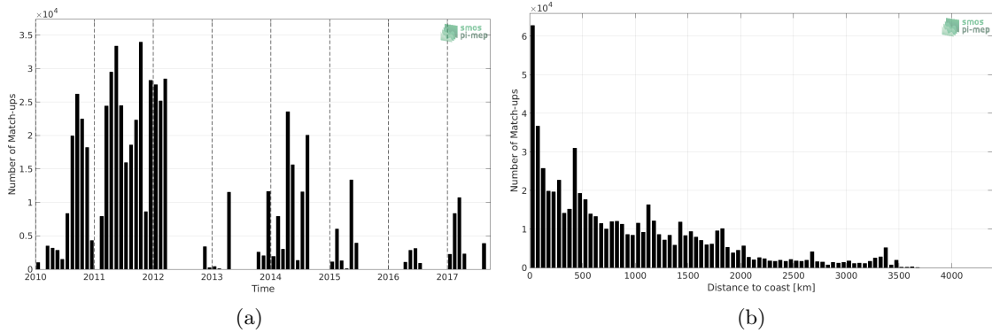
Figure 1: Number of match-ups between TSG (GOSUD-Sailing-ship) and SMOS SSS L3 v4 - 9 Days (CATDS-CECOS-LOCEAN) SSS as a function of time (a) and as function of the distance to coast (b) over the Mid-Low Latitudes 45N-45S Pi-MEP region and for the full satellite product period.
