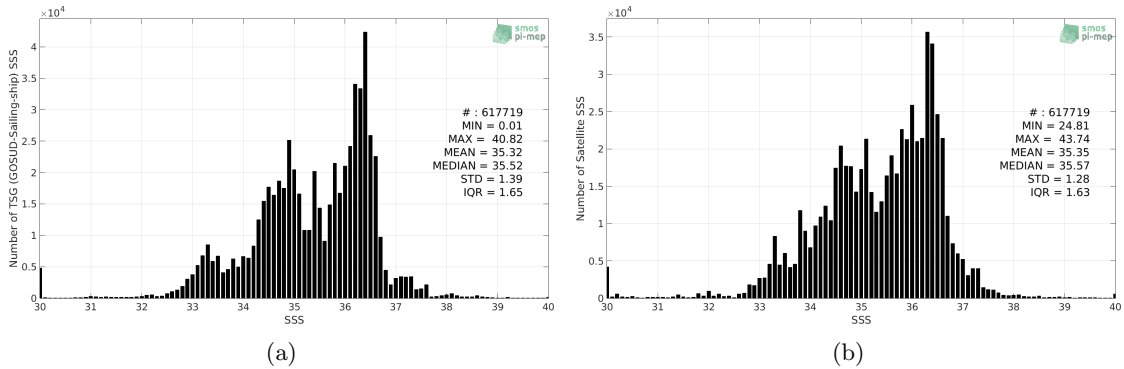
Figure 2: Histograms of SSS from TSG (GOSUD-Sailing-ship) (a) and SMOS SSS L3 v4 - 9 Days (CATDS-CECOS-LOCEAN) (b) considering all match-up pairs per bins of 0.1 over the Mid-Low Latitudes 45N-45S Pi-MEP region and for the full satellite product period.
