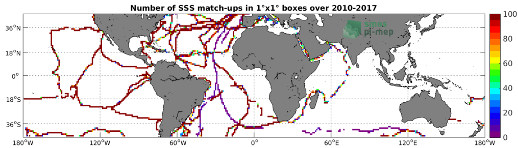
Figure 4: Number of SSS match-ups between TSG (GOSUD-Sailing-ship) SSS and the SMOS SSS L3 v4 - 9 Days (CATDS-CECOS-LOCEAN) SSS product for the Mid-Low Latitudes 45N-45S Pi-MEP region over 1^\circ \times 1^\circ boxes and for the full satellite product period.
