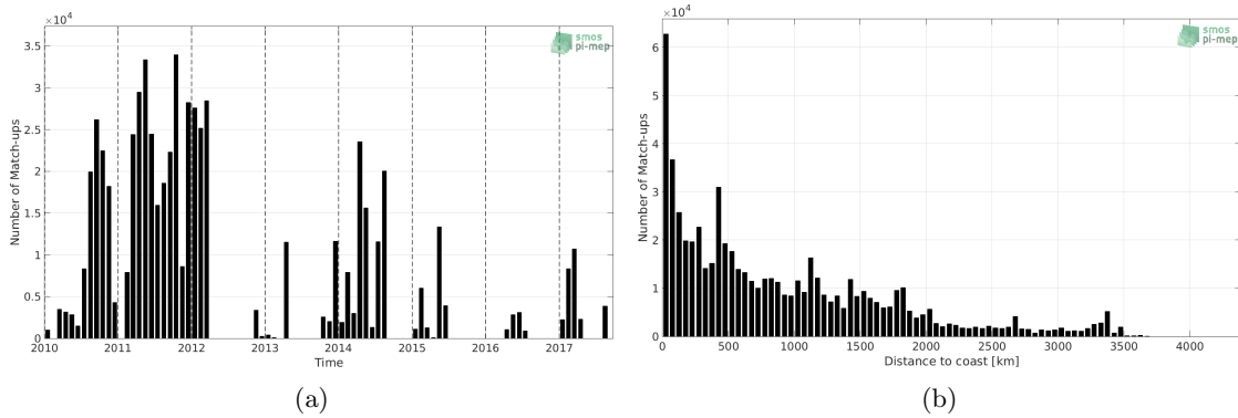
Figure 1: Number of match-ups between TSG-GOSUD-Sailing-ship and SMOS-L3-CATDS-CECOS-LOCEAN-V4-9DAYS-25KM SSS as a function of time (a) and as function of the distance to coast (b) over the Mid-Low Latitudes 45N-45S Pi-MEP region and for the full satellite product period.
