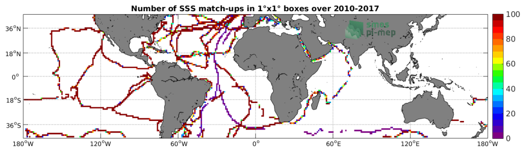
Figure 4: Number of SSS match-ups between TSG-GOSUD-Sailing-ship SSS and the SMOS-L3-CATDS-CECOS-LOCEAN-V4-9DAYS-25KM SSS product for the Mid-Low Latitudes 45N-45S Pi-MEP region over 1^\circ \times 1^\circ boxes and for the full satellite product period.
