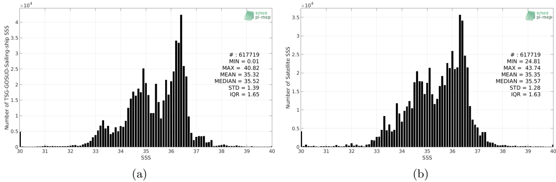
Figure 2: Histograms of SSS from TSG-GOSUD-Sailing-ship (a) and SMOS-L3-CATDS-CECOS-LOCEAN-V4-9DAYS-25KM (b) considering all match-up pairs per bins of 0.1 over the Mid-Low Latitudes 45N-45S Pi-MEP region and for the full satellite product period.
