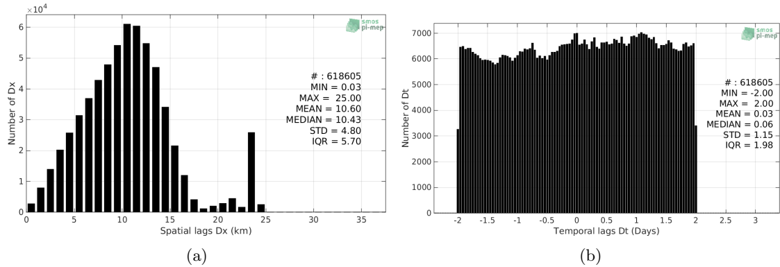
Figure 5: Histograms of the spatial (a) and temporal (b) lags between the time of the TSG-GOSUD-Sailing-ship measurements and the date of the corresponding SMOS-L3-CATDS-CECOS-LOCEAN-V4-9DAYS-25KM SSS product.
