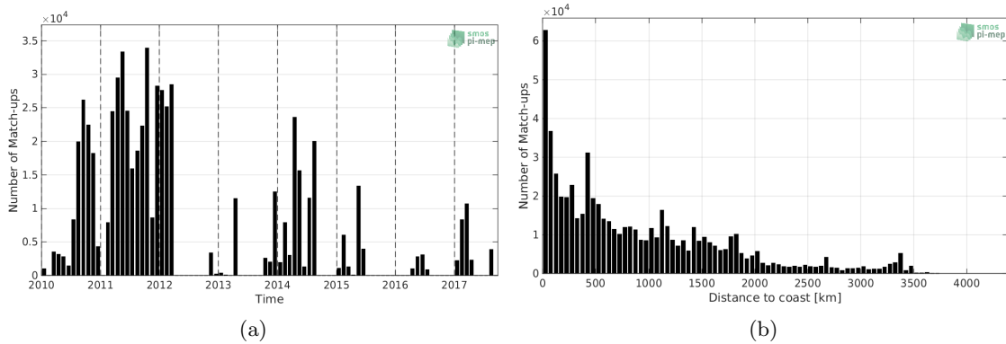
Figure 1: Number of match-ups between TSG-GOSUD-Sailing-ship and SMOS-L3-CATDS-CECOS-LOCEAN-V4-9DAYS-25KM SSS as a function of time (a) and as function of the distance to coast (b) over the Mid-Low Latitudes 45N-45S Pi-MEP region and for the full satellite product period.
