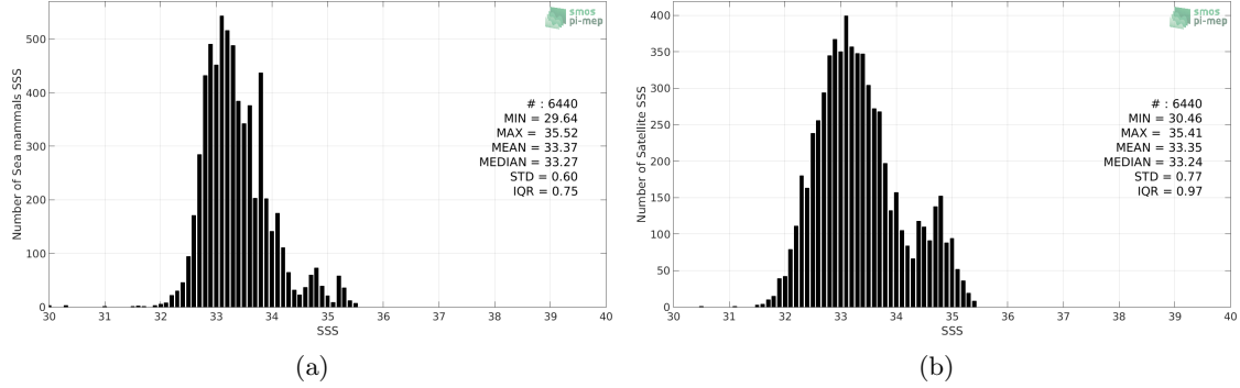
Figure 2: Histograms of SSS from Sea mammals (a) and SMOS SSS L3 v4 - 9 Days (CATDS-CECOS-LOCEAN) (b) considering all match-up pairs per bins of 0.1 over the Mid-Low Latitudes 45N-45S Pi-MEP region and for the full satellite product period.
