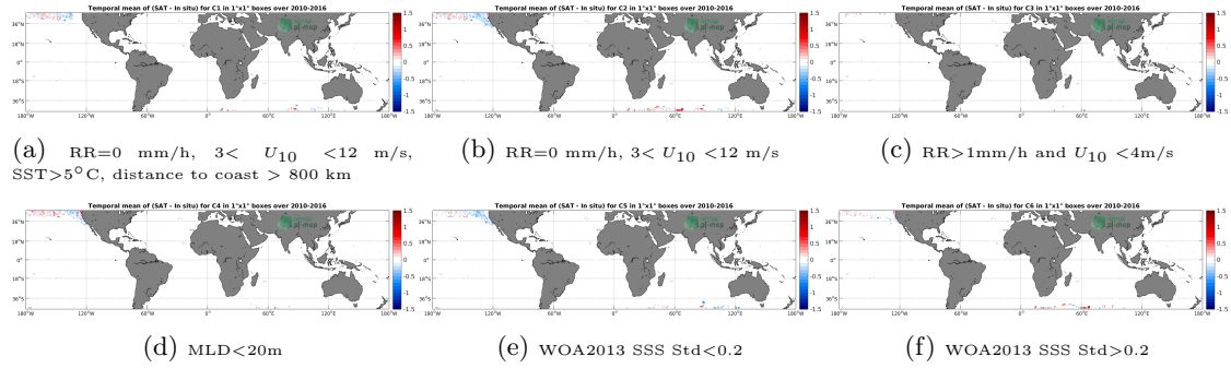
Figure 12: Temporal mean gridded over spatial boxes of size 1^\circ \times 1^\circ of \Delta SSS (SMOS SSS L3 v4 - 9 Days (CATDS-CECOS-LOCEAN) - Sea mammals) for 6 different subdatasets corresponding to: RR=0 mm/h, 3 < U_{10} < 12 m/s, SST > 5^\circ C , distance to coast > 800 km (a), RR=0 mm/h, 3 < U_{10} < 12 m/s (b), RR > 1 mm/h and U_{10} < 4 m/s (c), MLD < 20 m (d), WOA2013 SSS Std < 0.2 (e), WOA2013 SSS Std > 0.2 (f).
