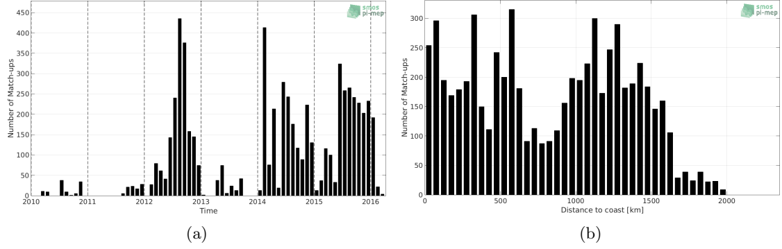
Figure 1: Number of match-ups between Sea mammals and SMOS SSS L3 v4 - 9 Days (CATDS-CECOS-LOCEAN) SSS as a function of time (a) and as function of the distance to coast (b) over the Mid-Low Latitudes 45N-45S Pi-MEP region and for the full satellite product period.
