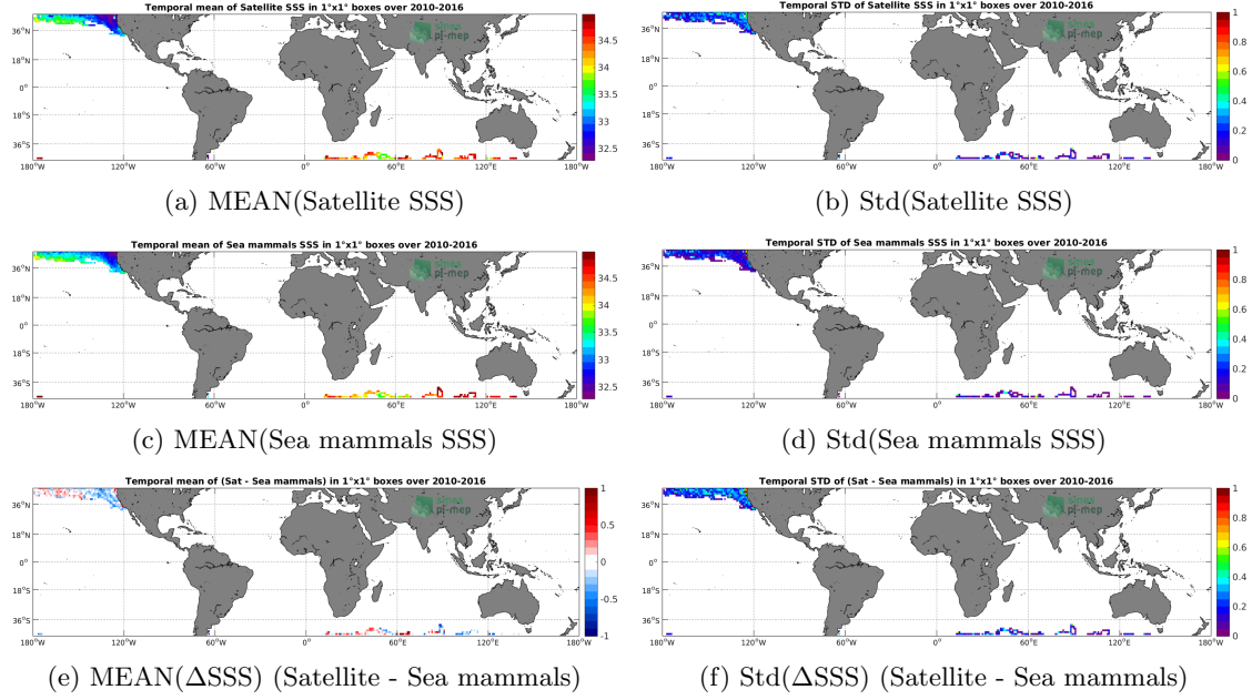
Figure 6: Temporal mean (left) and Std (right) of SSS from SMOS SSS L3 v4 - 9 Days (CATDS-CECOS-LOCEAN) (top), Sea mammals (middle), and of \Delta SSS (Satellite - Sea mammals). Only match-up pairs are used to generate these maps.
