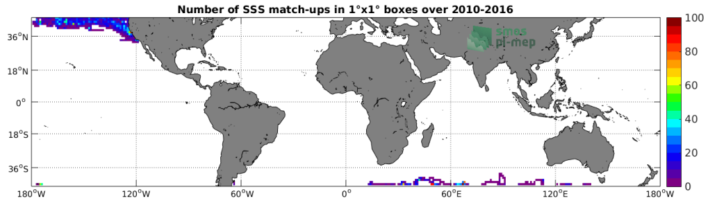
Figure 4: Number of SSS match-ups between Sea mammals SSS and the SMOS SSS L3 v4 - 9 Days (CATDS-CECOS-LOCEAN) SSS product for the Mid-Low Latitudes 45N-45S Pi-MEP region over 1°x1° boxes and for the full satellite product period.
