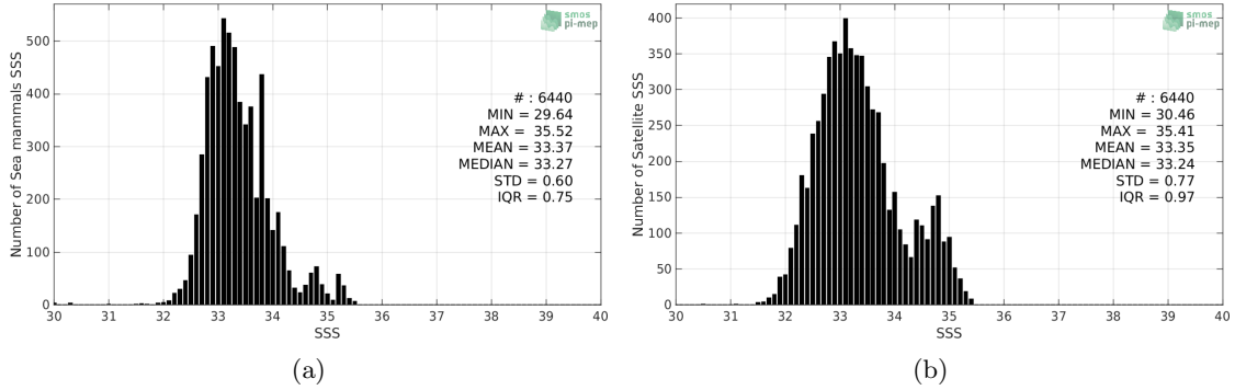
Figure 2: Histograms of SSS from Sea mammals (a) and SMOS-L3-CATDS-CECOS-LOCEAN-V4-9DAYS-25KM (b) considering all match-up pairs per bins of 0.1 over the Mid-Low Latitudes 45N-45S Pi-MEP region and for the full satellite product period.
