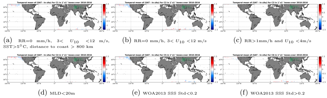
Figure 12: Temporal mean gridded over spatial boxes of size 1^\circ \times 1^\circ of \Delta SSS (SMOS-L3-CATDS-CECOS-LOCEAN-V4-9DAYS-25KM - Sea mammals) for 6 different subdatasets corresponding to: RR=0 mm/h, 3 < U_{10} < 12 m/s, SST >5^\circ\text{C} , distance to coast > 800 km (a), RR=0 mm/h, 3 < U_{10} < 12 m/s (b), RR >1 mm/h and U_{10} < 4 m/s (c),MLD <20 m (d),WOA2013 SSS Std <0.2 (e),WOA2013 SSS Std >0.2 (f).
