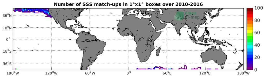
Figure 4: Number of SSS match-ups between Sea mammals SSS and the SMOS-L3-CATDS-CECOS-LOCEAN-V4-9DAYS-25KM SSS product for the Mid-Low Latitudes 45N-45S Pi-MEP region over 1°x1° boxes and for the full satellite product period.
