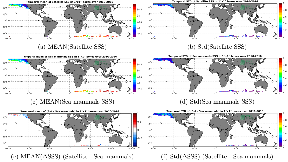
Figure 6: Temporal mean (left) and Std (right) of SSS from SMOS-L3-CATDS-CECOS-LOCEAN-V4-9DAYS-25KM (top), Sea mammals (middle), and of \Delta SSS (Satellite - Sea mammals). Only match-up pairs are used to generate these maps.
