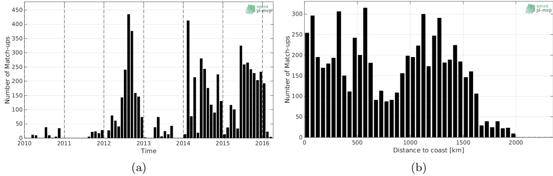
Figure 1: Number of match-ups between Sea mammals and SMOS-L3-CATDS-CECOS-LOCEAN-V4-9DAYS-25KM SSS as a function of time (a) and as function of the distance to coast (b) over the Mid-Low Latitudes 45N-45S Pi-MEP region and for the full satellite product period.
