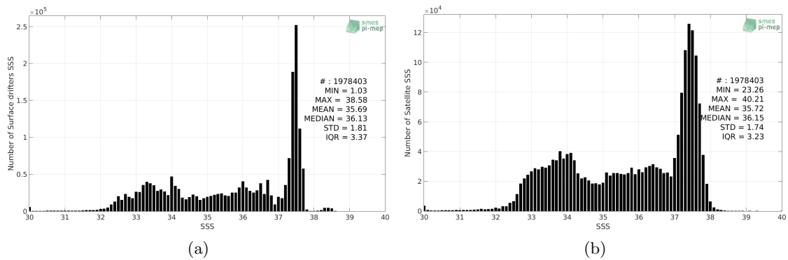
Figure 2: Histograms of SSS from Surface drifters (a) and SMOS SSS L3 v4 - 9 Days (CATDS-CECOS-LOCEAN) (b) considering all match-up pairs per bins of 0.1 over the Mid-Low Latitudes 45N-45S Pi-MEP region and for the full satellite product period.
