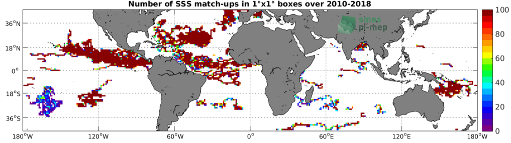
Figure 3: Number of SSS match-ups between Surface drifters SSS and the SMOS SSS L3 v4 - 9 Days (CATDS-CECOS-LOCEAN) SSS product for the Mid-Low Latitudes 45N-45S Pi-MEP region over 1°x1° boxes and for the full satellite product period.
