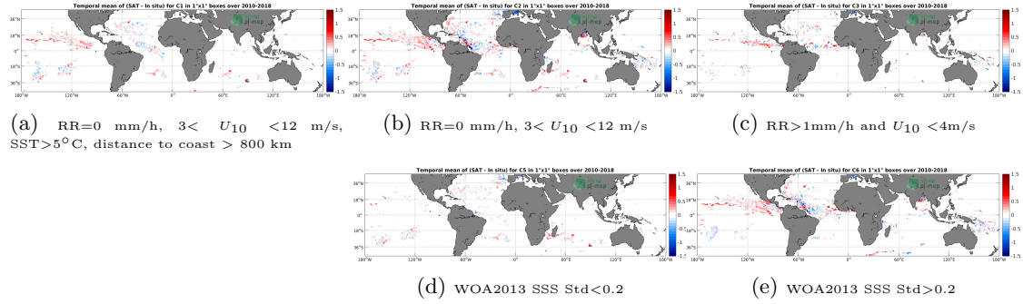
Figure 11: Temporal mean gridded over spatial boxes of size 1^\circ \times 1^\circ of \Delta SSS (SMOS SSS L3 v4 - 9 Days (CATDS-CECOS-LOCEAN) - Surface drifters) for 5 different subdatasets corresponding to: RR=0 mm/h, 3 < U_{10} < 12 m/s, SST > 5^\circ C , distance to coast > 800 km (a), RR=0 mm/h, 3 < U_{10} < 12 m/s (b), RR > 1 mm/h and U_{10} < 4 m/s (c), WOA2013 SSS Std < 0.2 (d), WOA2013 SSS Std > 0.2 (e).
