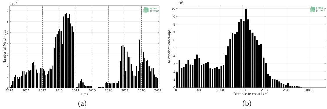
Figure 1: Number of match-ups between Surface drifters and SMOS SSS L3 v4 - 9 Days (CATDS-CECOS-LOCEAN) SSS as a function of time (a) and as function of the distance to coast (b) over the Mid-Low Latitudes 45N-45S Pi-MEP region and for the full satellite product period.
