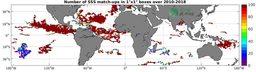
Figure 3: Number of SSS match-ups between Surface drifters SSS and the SMOS-L3-CATDS-CECOS-LOCEAN-V4-9DAYS-25KM SSS product for the Mid-Low Latitudes 45N-45S Pi-MEP region over 1°x1° boxes and for the full satellite product period.
