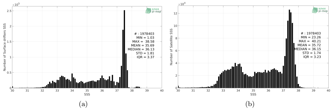
Figure 2: Histograms of SSS from Surface drifters (a) and SMOS-L3-CATDS-CECOS-LOCEAN-V4-9DAYS-25KM (b) considering all match-up pairs per bins of 0.1 over the Mid-Low Latitudes 45N-45S Pi-MEP region and for the full satellite product period.
