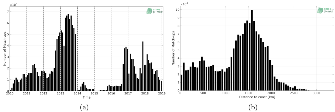
Figure 1: Number of match-ups between Surface drifters and SMOS-L3-CATDS-CECOS-LOCEAN-V4-9DAYS-25KM SSS as a function of time (a) and as function of the distance to coast (b) over the Mid-Low Latitudes 45N-45S Pi-MEP region and for the full satellite product period.
